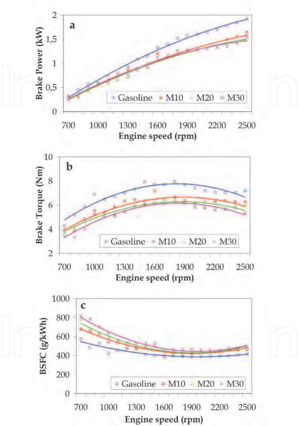
Fig. 3. Experimental results of engine performance characteristics using different methanol gasoline blended fuels under various engine speeds. (a) Brake power, (b) Brake torque, and (c) Brake specific fuel consumption.
