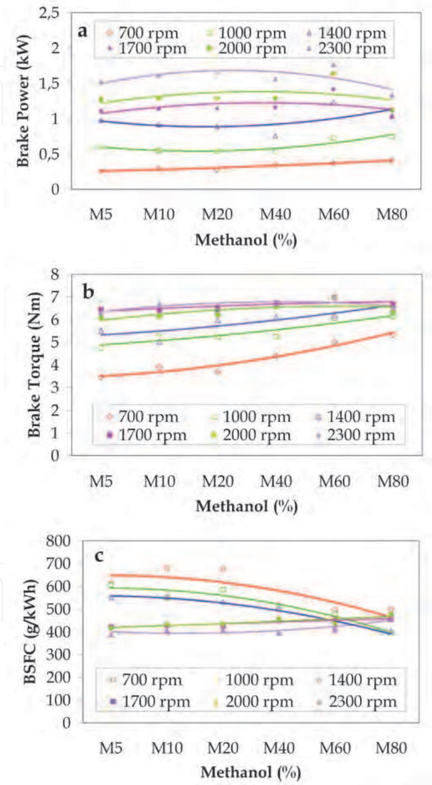
Fig. 5. The influence of methanol addition on the engine performance characteristics. (a) Brake power, (b) Brake torque, and (c) Brake specific fuel consumption.
