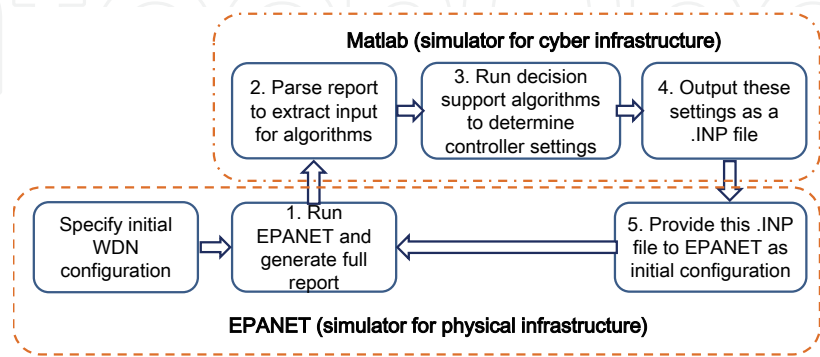
Fig. 6. Procedure for simulation of an intelligent WDN
