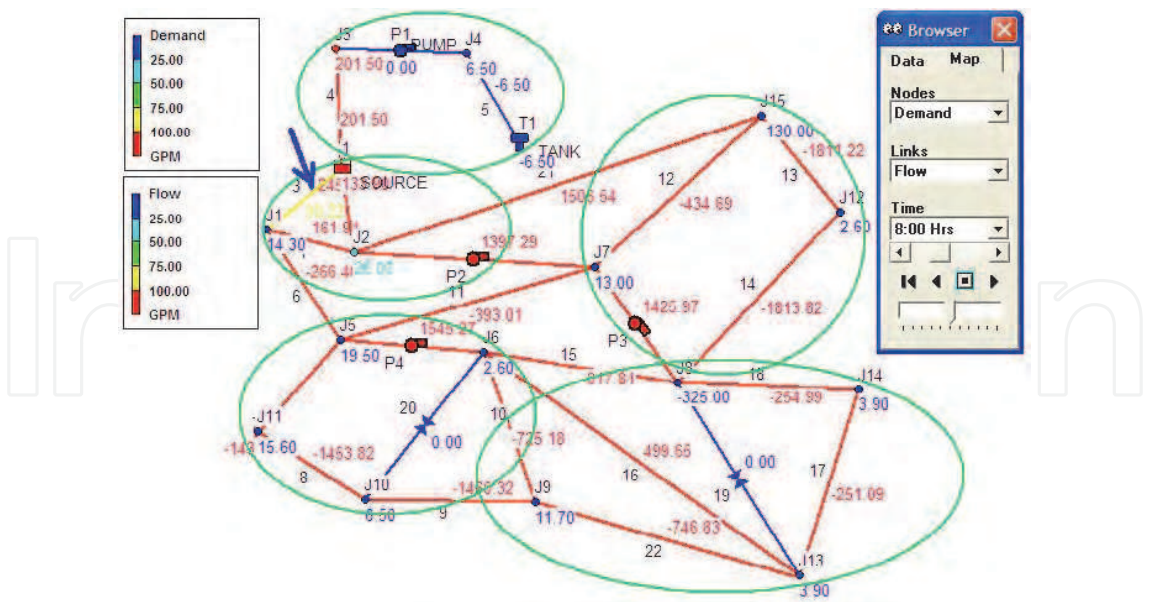
Fig. 3. A more complex topology and node groupings in EPANET
