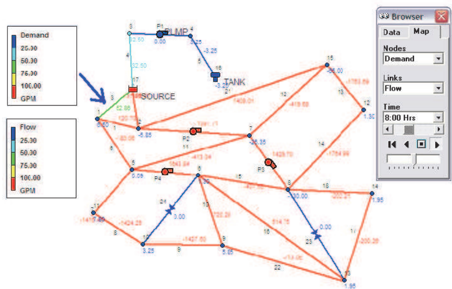
Fig. 8. Complex topology after applying cyber control
