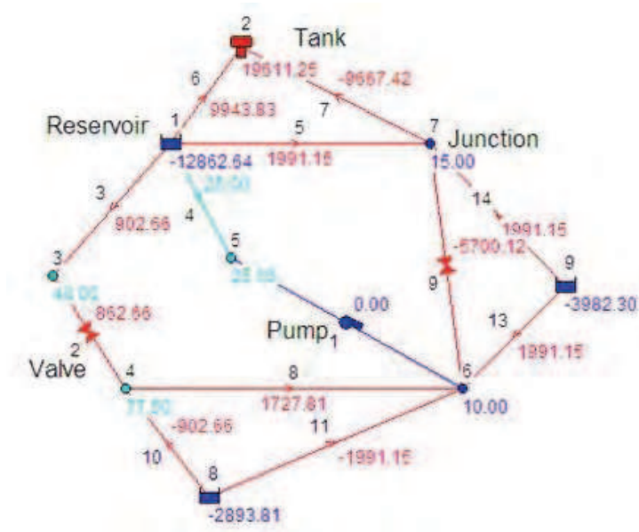
Fig. 16. Topology of simulation for all reservoirs are serving.
