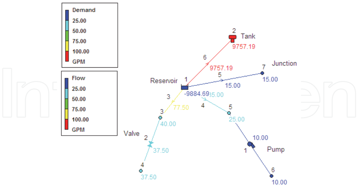
Fig. 2. A simple topology in EPANET
