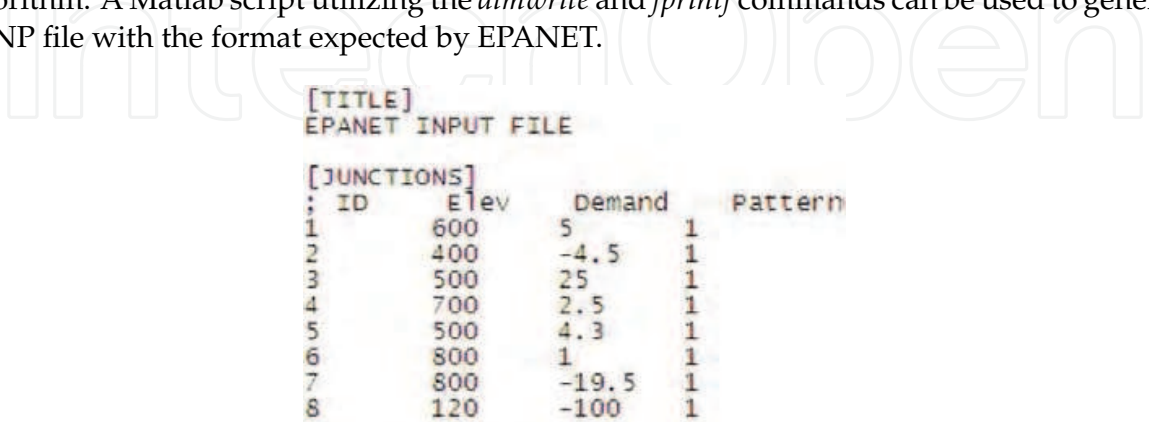
Fig. 7. EPANET input file generated by MATLAB
