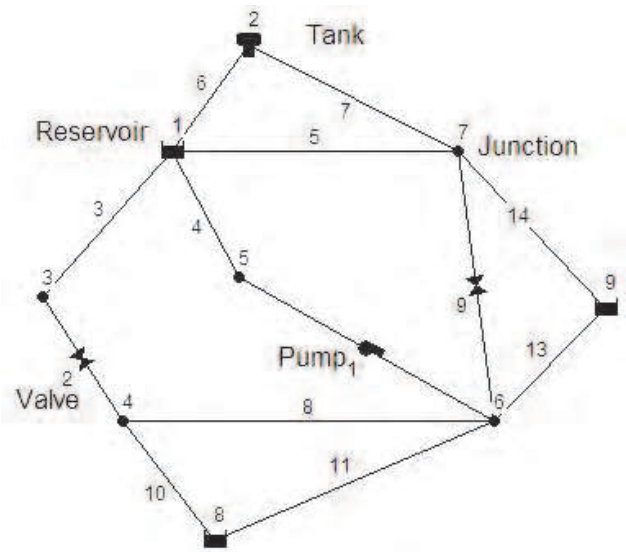
Fig. 10. Simple topology for integrating game theory.
