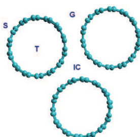
Fig. 8. Smaller simulation cluster, showing adsorption sites: the grooves (G) between two tubes; on nanotube surface (S); in interstitial channels (IC); and in the interior of a nanotube (T), for open tubes. (Adapted from Albessa et al., 2010) Copyright 2010 American Chemical Society
