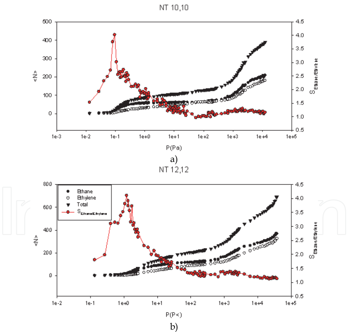
Fig. 22. Isotherms and Selectivity (right offset) for ethane/ethylene as a function of the pressure in a) (10,10) nanotubes b) in (12,12) nanotubes
