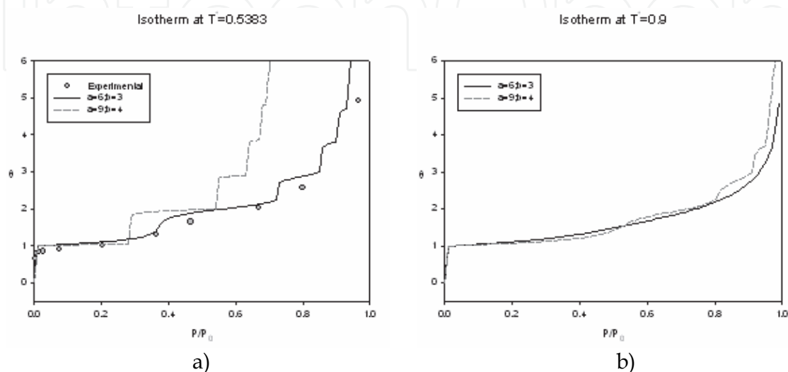
Fig. 5. Experimental and lattice gas model isotherms at (a)103 K.(b) Experimental and lattice gas model isotherms at 171 K. (Adapted from Albessa et al., 2008) Copyright 2008 American Chemical Society
