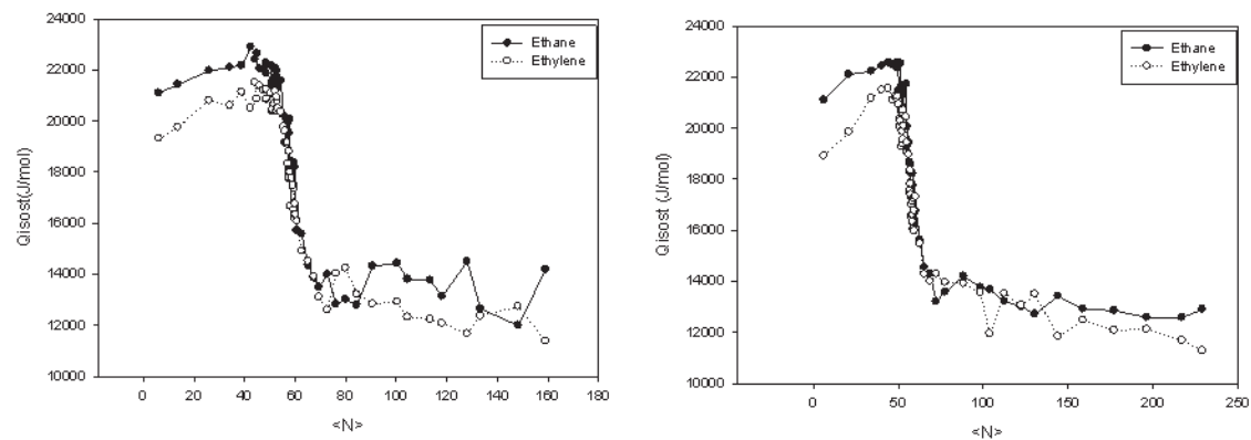
Fig. 20. Isosteric heat of adsorption at 153 K for ethane/ethylene mixtures on graphite for different compositions (a) 25%Ethane (b)75%Ethane
