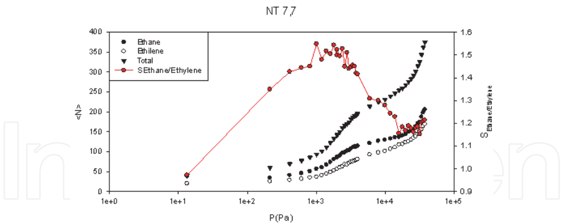
Fig. 21. Isotherms and Selectivity (right offset) for ethane/ethylene in (7,7) nanotubes as a function of the pressure
