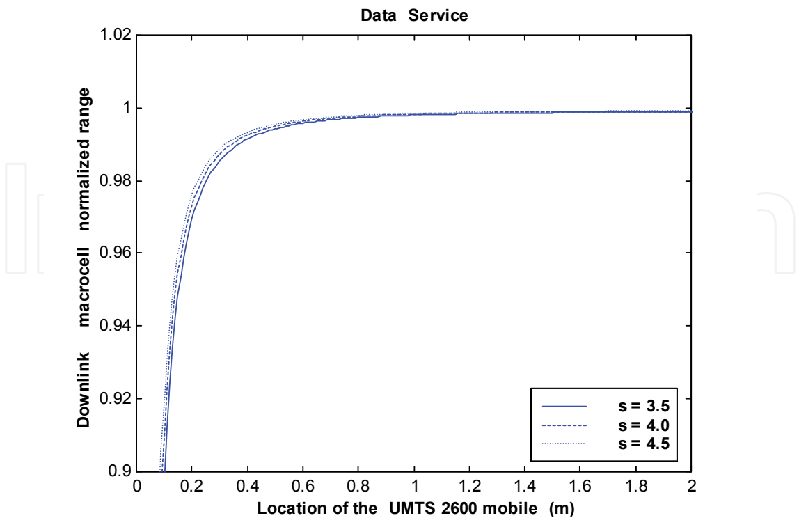
Fig. 12. Effect of the UWB interference on the macrocell range as a function of the UMTS2600 mobile location ( P_{UWB} = -82 dBm/MHz) for multi UWB transmitters and 9.5 dB noise rise.
