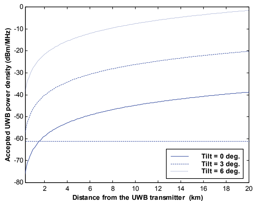
Fig. 6. Maximum permitted UWB EIRP for an outdoor environment for three RADAR antenna tilt (UWB antenna height = 30m and RADAR antenna height = 30m). Here we address the effect of the UWB system on the downlink of the UMTS2600 system. In the analysis we assume that the UWB data rate is higher than the UMTS2600 chip rate, i.e., the UWB bit rate is higher than 4 Mbps. In Fig. 7, the UWB interference power on the UMTS2600 downlink (i.e. interference as seen at the mobile) is plotted assuming an average P_{UWB} of -51.3 dBm/MHz within the UMTS2600 bandwidth.
