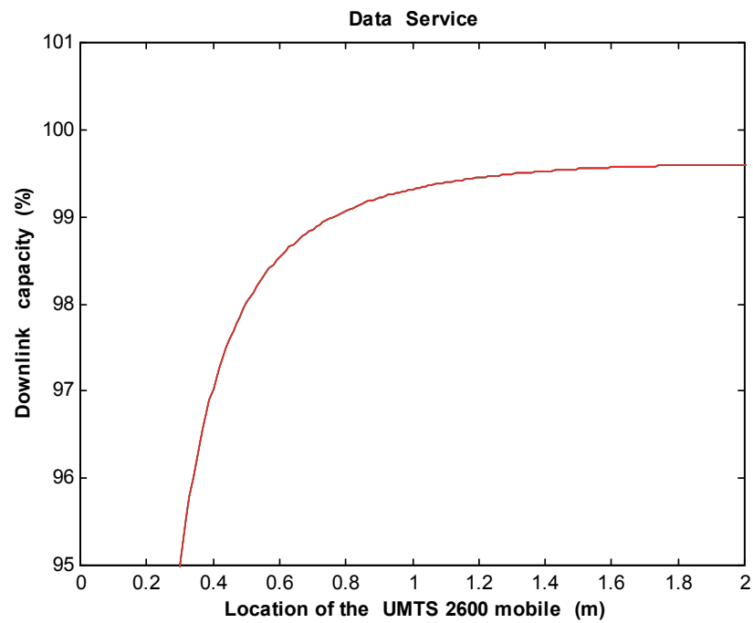
Fig. 13. Effect of the UWB interference on the macrocell normalized capacity as a function of the UMTS2600 mobile location ( P_{UWB} = -82 \text{ dBm/MHz} ) for multi UWB transmitters and 9.5 dB noise rise.
