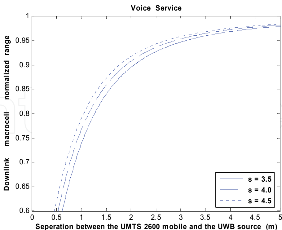
Fig. 8. Effect of the UWB interference on the macrocell range as a function of the separation between the UWB transmitter and the UMTS2600 mobile ( P_{\text{UWB}} = -51.3 dBm/MHz).
