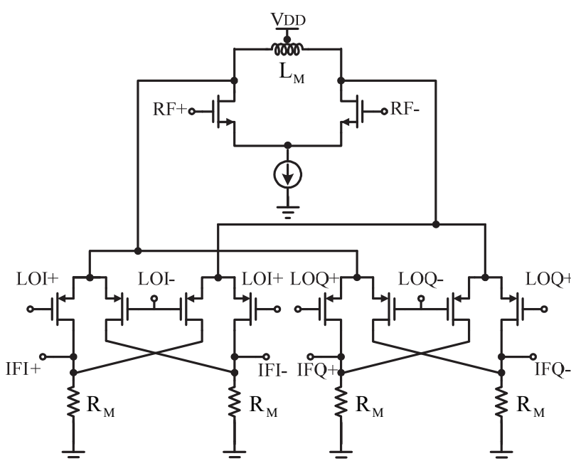
Fig. 5. Quadrature down conversion mixer circuit
