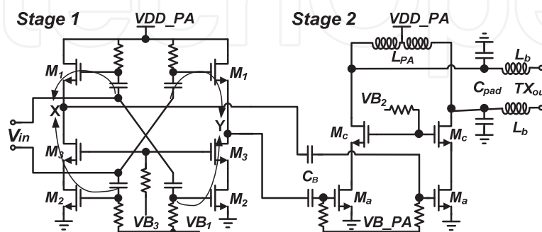
Fig. 12. Simplified schematic of two-stage PA
