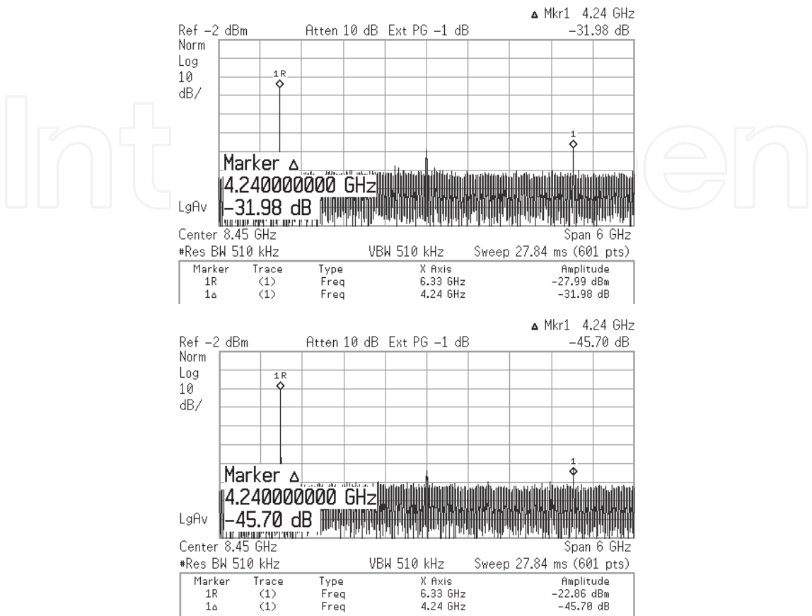
Fig. 24. Output spectrum of 6336 MHz (up) without calibration and (down) with calibration
