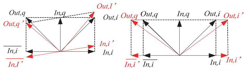
Fig. 19. Illustration of the phase and gain mismatch translation
