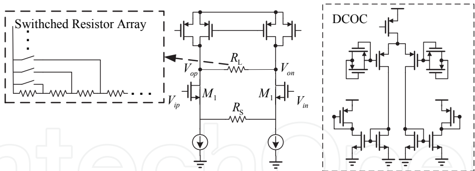
Fig. 8. Topology of the PGA
