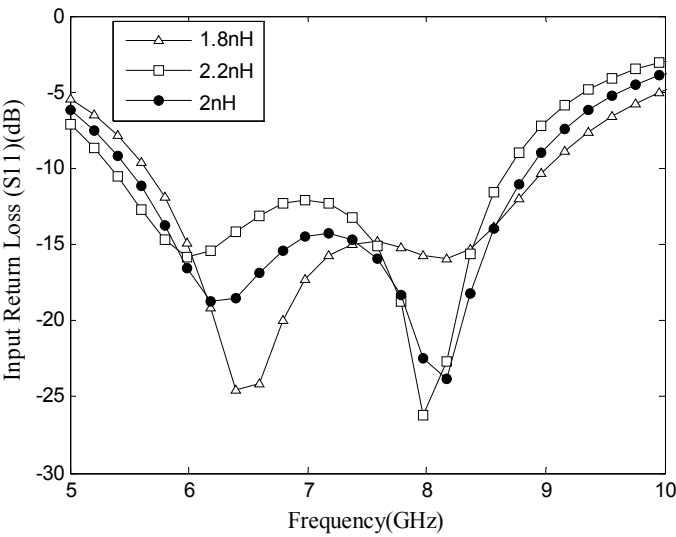
Fig. 4. Simulated S11 with different bonding wire inductance
