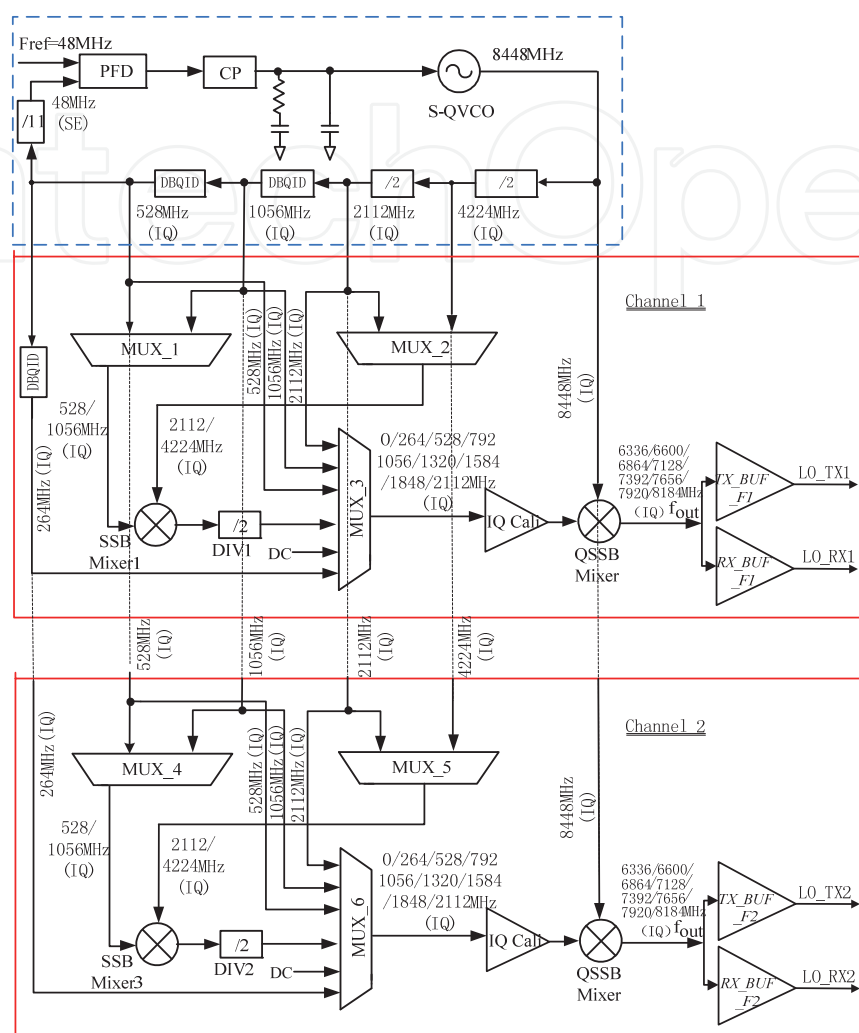
Fig. 13. Architecture of the proposed frequency synthesizer
