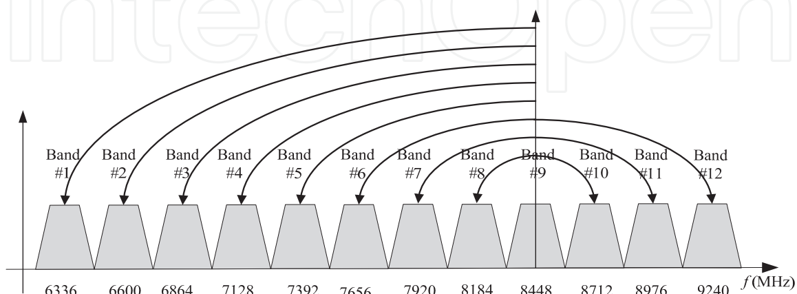
Fig. 14. Frequency plan of the proposed frequency synthesizer
