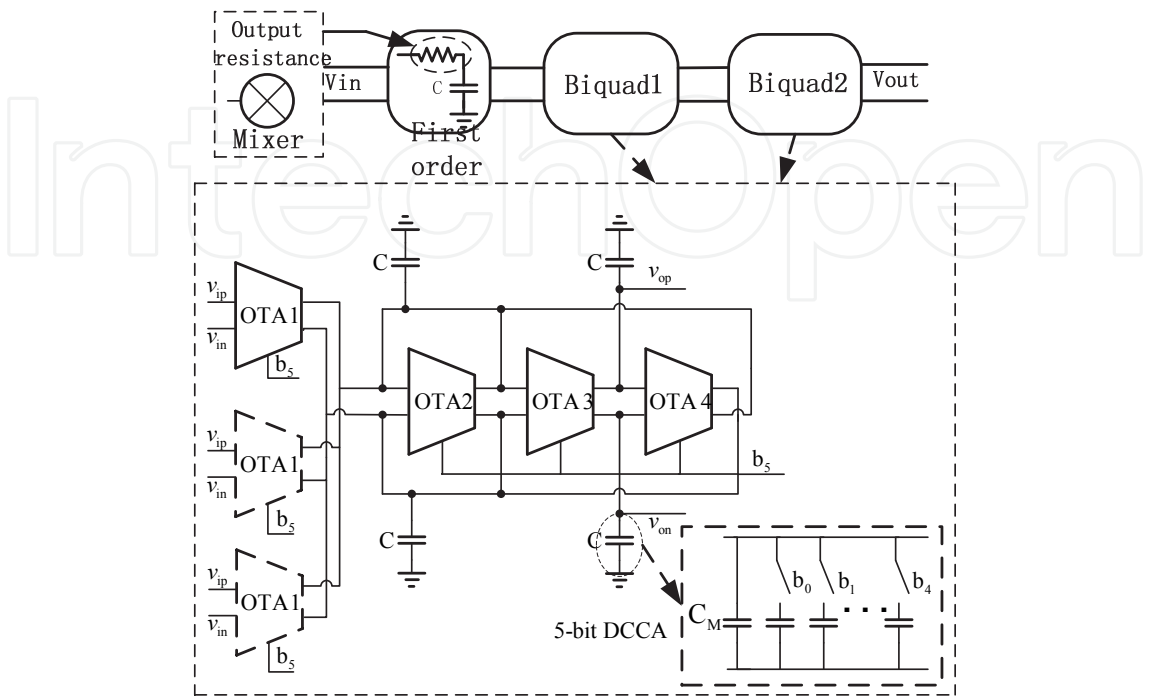
Fig. 6. Structure of the Low Pass Filter
