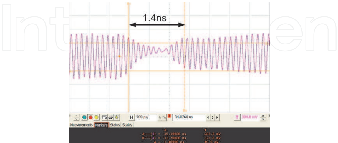
Fig. 25. Measured band switching behaviour
