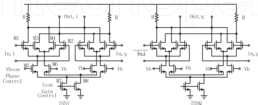
Fig. 18. Schematic of the IQ calibration
