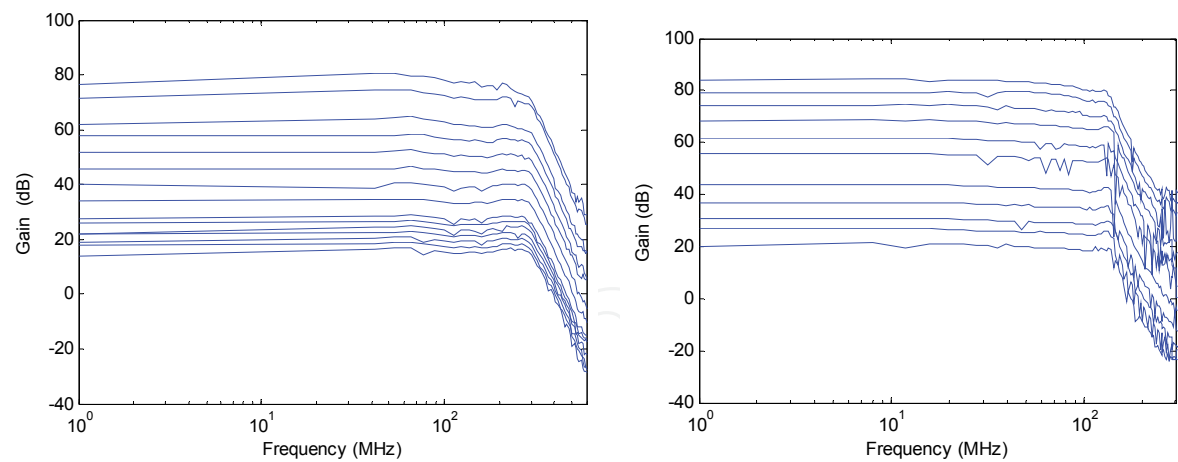
Fig. 21. Receiver frequency response, (left) At cut-off frequency of 264MHz; (right) At cut-off frequency of 132MHz
