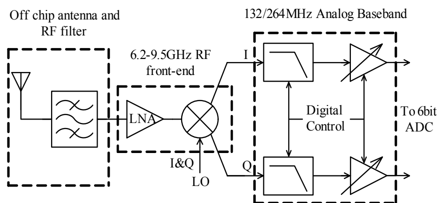
Fig. 2. Architecture of the proposed receiver
