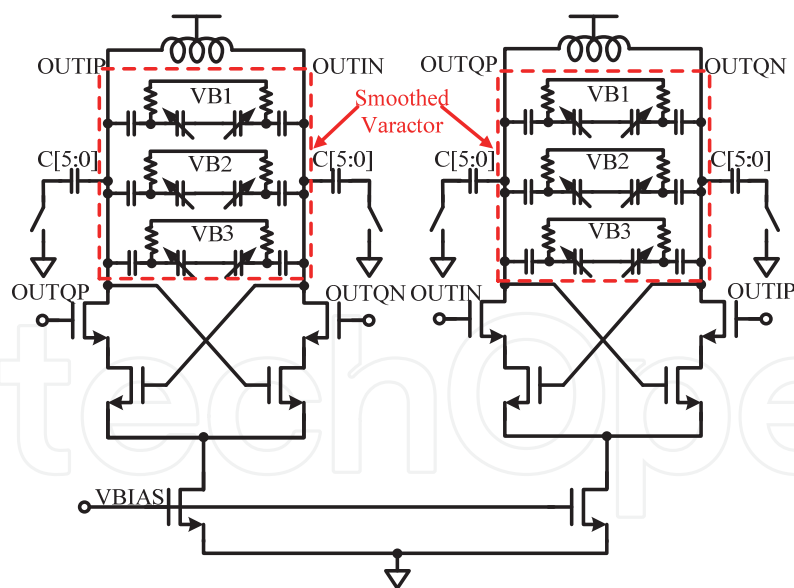
Fig. 15. Schematic of TS-QVCO
