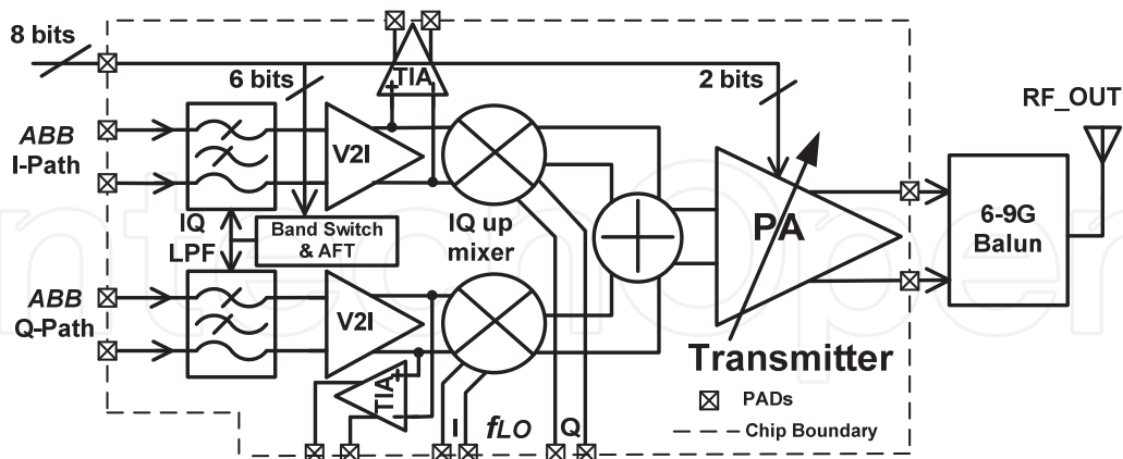
Fig. 9. Block diagram of the proposed transmitter
