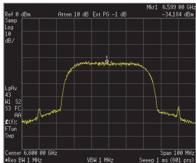
Fig. 22. Spectrum mask of the transmitter with 40MHz QPSK modulation signal
