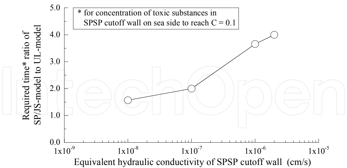
Fig. 12. Required time ratio of both models, for concentration of toxic substances in SPSP cutoff wall on sea side to reach C = 0.1 , with equivalent hydraulic conductivity of SPSP cutoff wall
