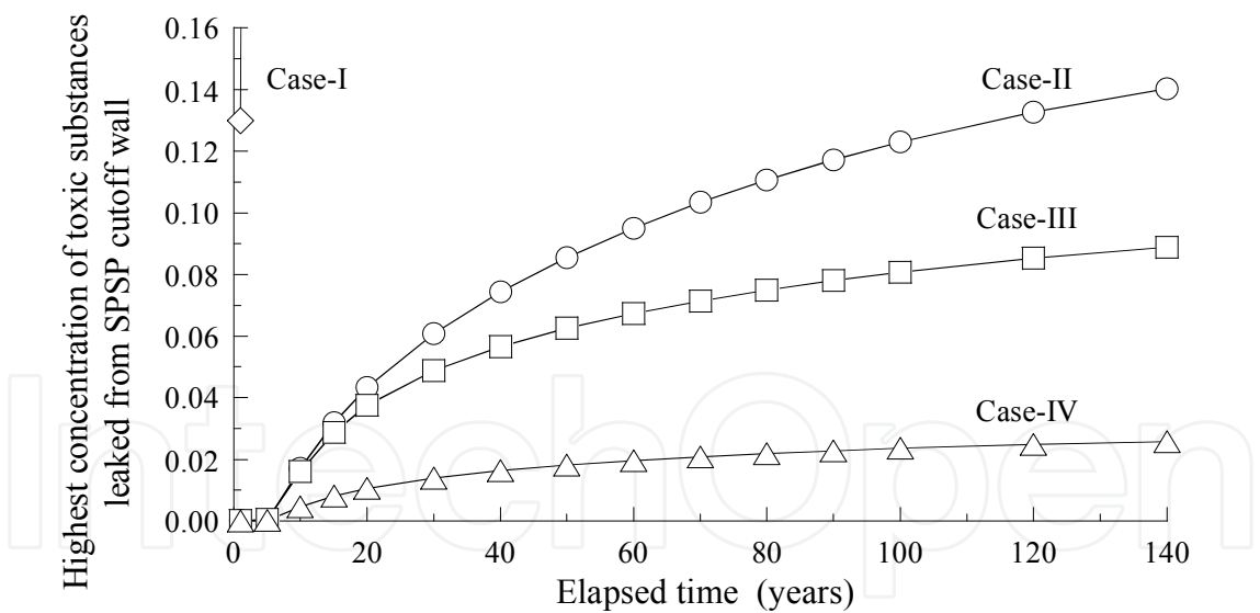
Fig. 15. Relationships between elapsed time and the highest concentration of toxic substances leaked from SPSP cutoff wall onto sea side for Case-I to Case-IV
