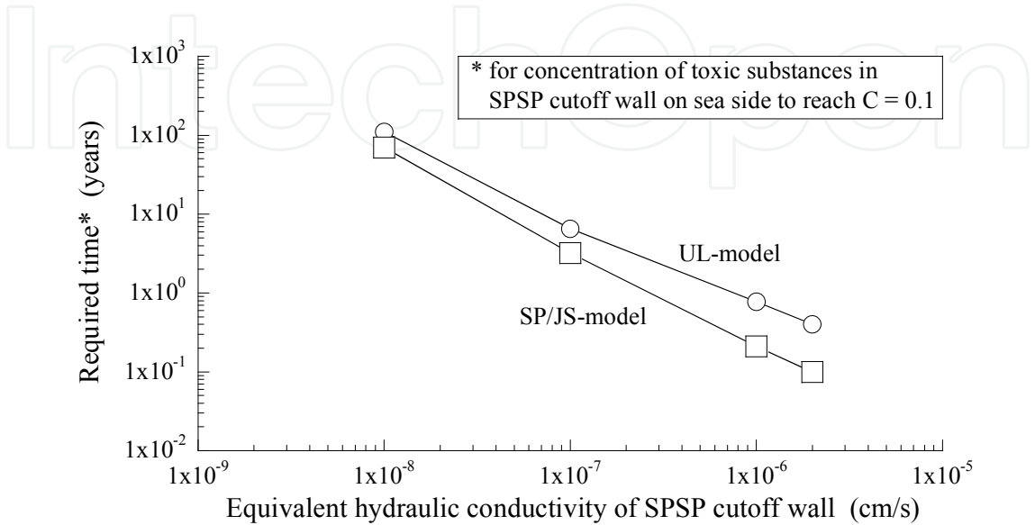
Fig. 11. Required time for concentration of toxic substances in SPSP cutoff wall on sea side to reach C = 0.1 with equivalent hydraulic conductivity of SPSP cutoff wall
