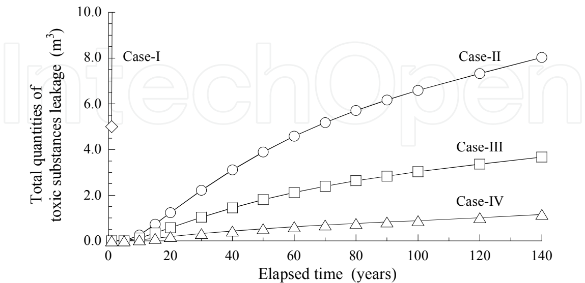
Fig. 14. Total quantities of toxic substances leaked from SPSP cutoff wall onto sea side with respect to the elapsed time for Case-I to Case-IV
