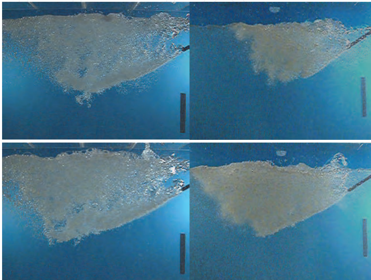
Fig. 10. The diphase stream injection for the particles of d_c=0.833 mm diameter and \rho=882 kg/m 3 density, liquid density \rho_{\text{osr}}=1000 kg/m 3 (left) and \rho_{\text{osr}}=1180 kg/m 3 (right picture)
