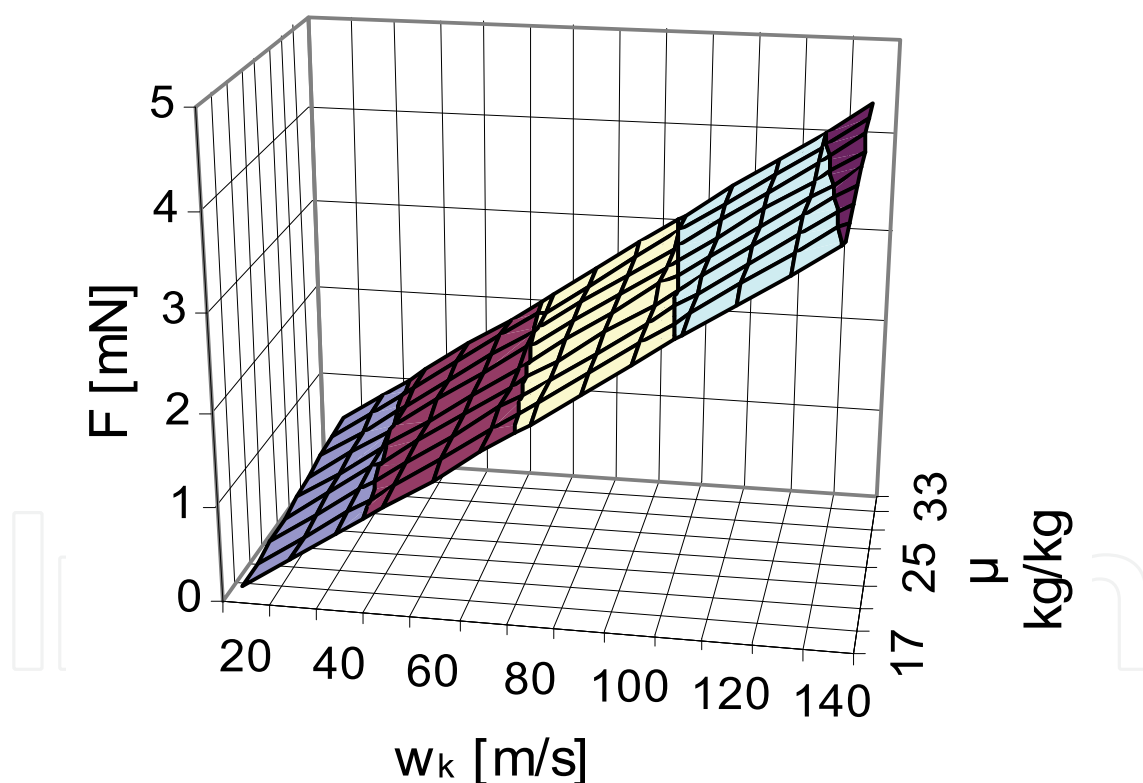
Fig. 16. Influence of gas velocity in lance outlet and mass concentration on the stream force ( d_w = 6.1\text{mm} , H = 10\text{mm} )
