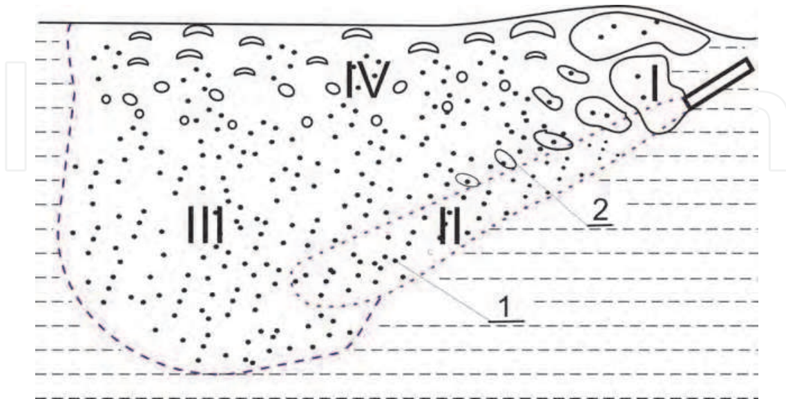
Fig. 11. The shape and area of the diphase stream: 1-carburizer particles, 2-gas bubbles
