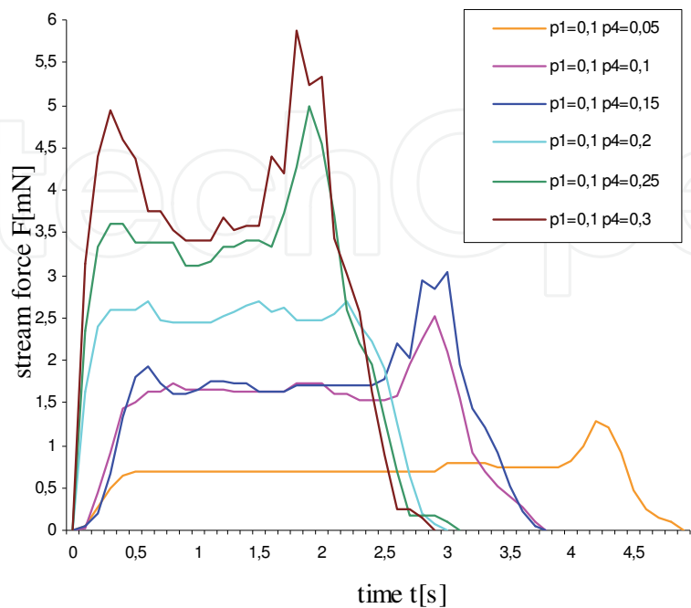
Fig. 14. Diphas stream force character for parameters as follows: lance diameter d_w = 6.1\text{mm} , distance between lance outlet and measuring device’s surface H = 40\text{mm} , carrier gas pressure p_1 = 0.1\text{MPa} , powdered material – polyethylene of granulation 0.4mm
