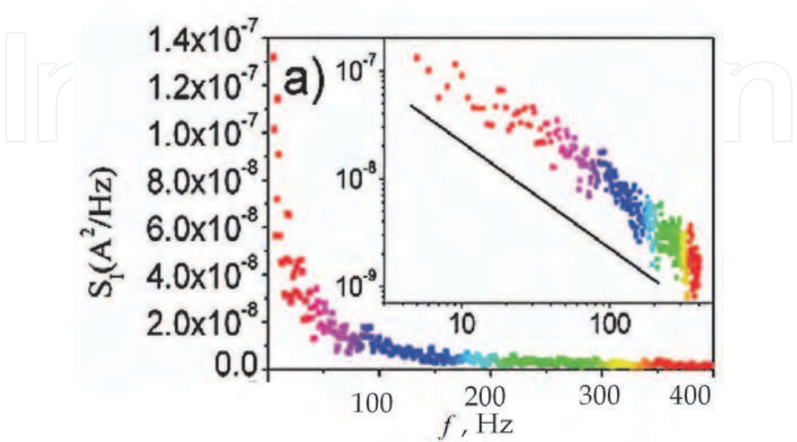
Fig. 5. Spectrum of 1/f -noise for a CNT FET at a bias voltage of 100 mV with each frequency point color coded a gate voltage of -8V, and a T=150 K, shown on linear-linear scale (main panel) and log-log scale (inset). The solid line in the inset indicates a slope of -1 (Tobias et al., 2008).
