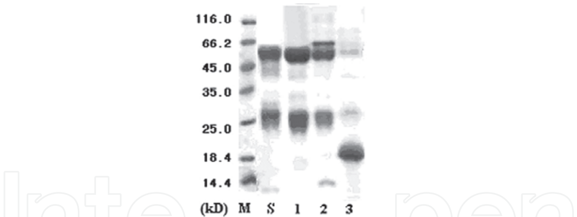
Fig. 6. SDS-PAGE profile of fractions obtained in ultrafiltrated whey by anion-exchange chromatography using saline gradient. Lane M, proteins marker; lane S, IgG standard; lane 1, elution peak with 51 mmol/L NaCl; lane 2, elution peak with 103 mmol/L NaCl; lane 3, elution peak with 205 mmol/L NaCl with stepwise saline gradient.
