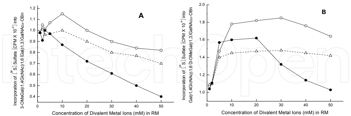
A. Case 7 tumor specimen; B. Case 3 tumor specimen ● Mn;Δ Mg; ○ Ca Fig. 1. Influence of divalent metal ions on gastric tumor Gal3 Sulfotransferase activities.
