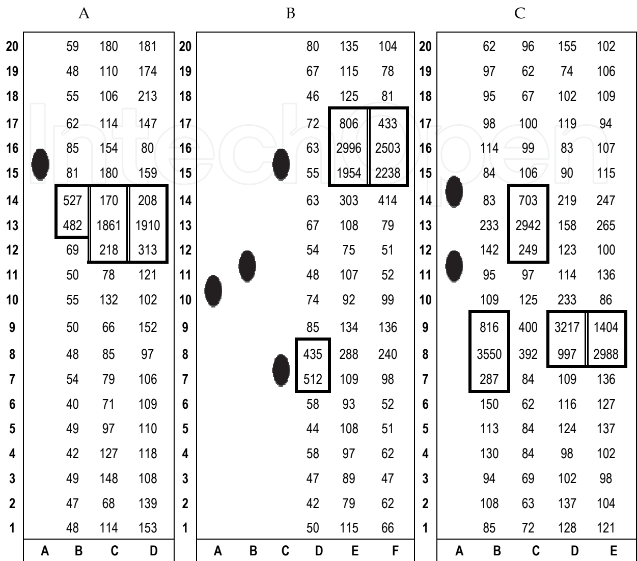
Fig. 2. TLC Identification of \beta GlcNAc: \alpha GlcNAc transferase activity in human gastric tumor Fig. 2 A (solvent system A). A: Acceptor compound 3-O-Me Gal \beta 1, 3 (GlcNAc \beta 1, 6) GalNAc \alpha -O-Bn B: [6- ^3 H] GlcNAc containing product resulting from A C and D: B incubated with and without \beta N-acetylhexosaminidase (Jack bean) Fig. 2. B (solvent system B). A: 3-O-Me Gal \beta 1, 3 (GlcNAc \beta 1, 6) GalNAc \alpha -O-Bn B: 3-O-Me Gal \beta 1, 3 (Gal \beta 1, 4 GlcNAc \beta 1, 6) GalNAc \alpha -O-Bn C: 3-O-Sulfo Gal \beta 1, 3 (Gal \beta 1, 4 GlcNAc \beta 1, 6) GalNAc \alpha -O-Bn and Std. GlcNAc D, E and F: [6- ^3 H] GlcNAc containing products resulting from A, B and C respectively after \beta N- acetylhexosaminidase(Jack bean) treatment Fig. 2. C (Solvent system B). A: The acceptor Gal \beta 1, 3 (GlcNAc \beta 1, 6) GalNAc \alpha -O-Al and Std. GlcNAc B: [6- ^3 H] GlcNAc containing product resulting from the acceptor in A C: B after \beta 1, 3 galactosidase (recombinant) treatment D and E: B incubated with and without \beta N- acetylhexosaminidase (Jack bean)
