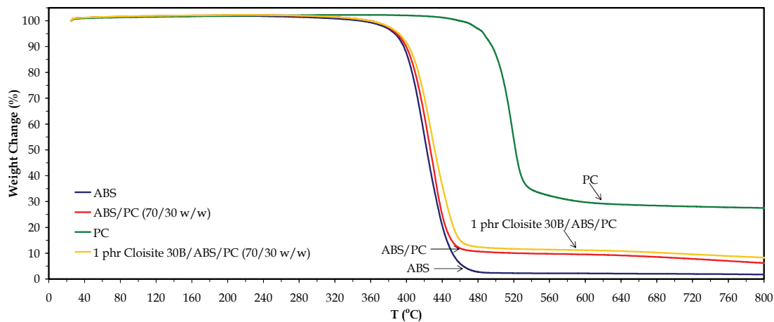
Fig. 8. TGA curves of ABS, PC, of ABS/PC (70/30 w/w) blend and 1 phr Cloisite 30B/ABS/PC (70/30 w/w) nanocomposite.
