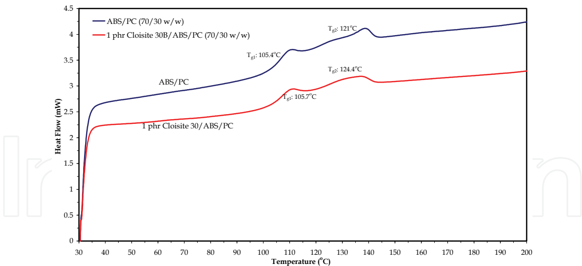
Fig. 7. DSC curves of ABS/PC (70/30 w/w) and 1 phr Cloisite 30B/ABS/PC (70/30 w/w) composite.
