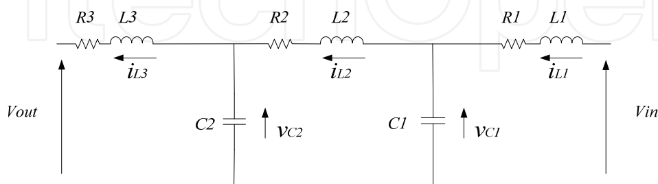
Fig. 12. Mono-phase representation of the transmission system with the submarine cable modeled as a unique “π” circuit
