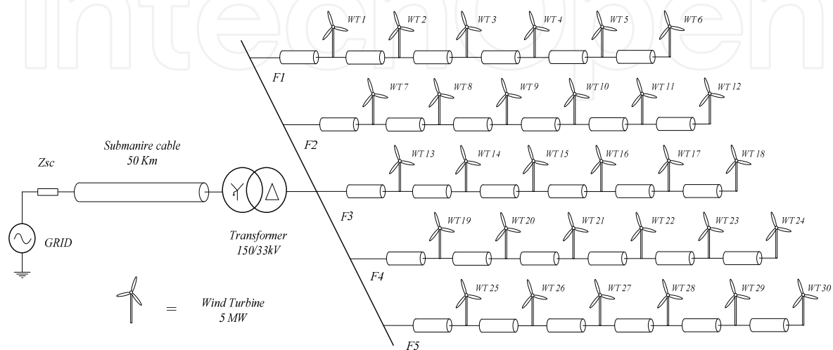
Fig. 15. The lay-out of the offshore wind farm, which is the base of the resonances analysis Considering that the transmission system is equal to the characterized in section 3.1, the last feature to define the whole offshore wind farm is the inter-turbine submarine cable. Hence, as inter-turbine submarine cable an ABB XLPE cable (Asea Brown Boveri [ABB], 2005) with the adequate nominal voltage and power is chosen. The characteristics of this cable are shown in Table 7.
