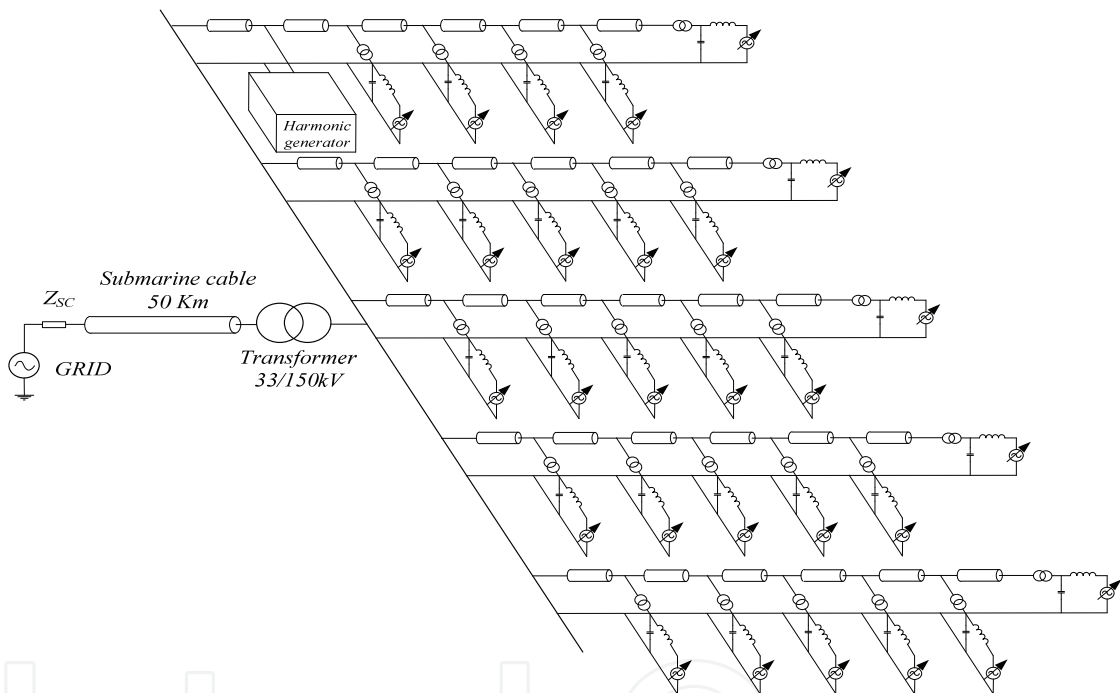
Fig. 16. Simulation scenario of the offshore wind farm, which is the base for the frequency response analysis Taking the scenario depicted in Fig. 16 as base to estimate the frequency response, the same procedure of section 3.1 is used. In this way, to know the frequency response for a specific wind turbine, it is substituted by a harmonic voltage generator (Fig. 16), which generates a harmonic train in the frequency range of 50Hz-5000Hz, Fig. 6.
