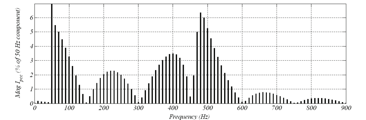
Fig. 9. Frequency response of the transmission system with a leakage inductance of 3% of the step-up transformer
