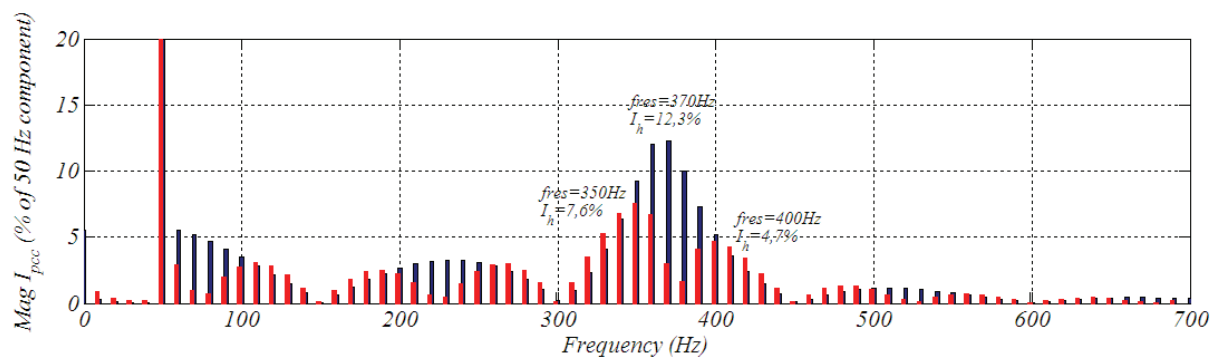
Fig. 22. Harmonic currents at the PCC: With 2 feeders F1-F2 (red) and with 2 feeders on each primary winding F1-F2 and F1'-F2' (black) Looking at the results in Fig. 22, it is possible to see that the use of two windings connected as delta-star(grounded)-delta, where the secondary windings have delta connection, does not allow to transmit multiples of 3 rd order divided by two harmonics (multiples of 150Hz/2, 75 Hz) to the PCC. As a result, the frequency response of the system from the viewpoint of the wind turbine presents less harmonic components. However, as can be seen in Fig. 23 (b), for the voltage harmonics, there is a new group of frequencies less attenuated at 2520 Hz.
