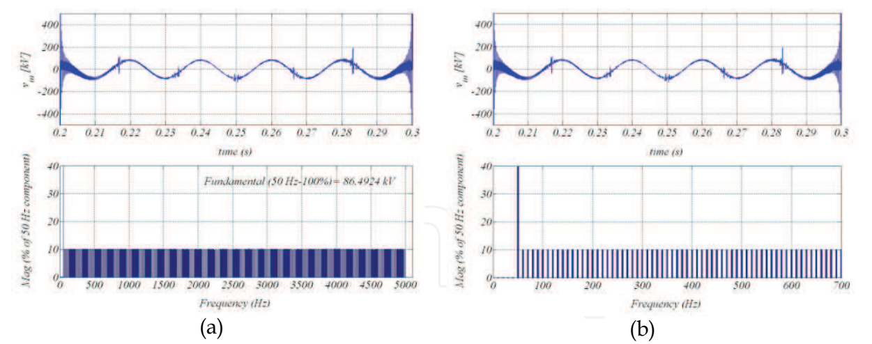
Fig. 6. Harmonic voltage train applied to the submarine cable model (resolution 10 Hz)
