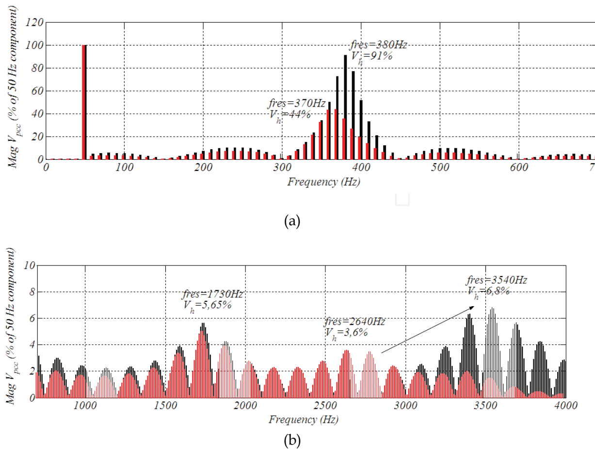
Fig. 18. Harmonic voltages at the PCC in function of the location of the harmonic voltage source inside the inter turbine grid. For the 25 th wind turbine (black) and for the 30 th wind turbine (red): (a) more detail in the main resonance and (b) more detail in high frequencies
