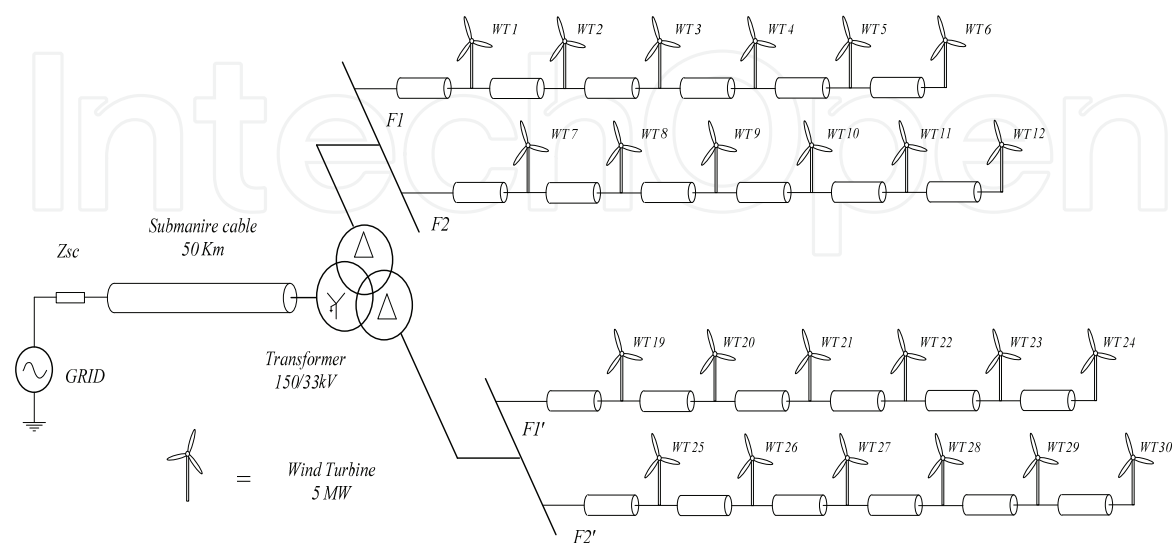
Fig. 21. Simplified scheme of the simulation scenario of the offshore wind farm with two primary windings To know the influence of the extra winding, the results of the configuration depicted in Fig. 21 and the configuration depicted in Fig. 15 with only two feeders, are compared. The comparison these frequency responses are served Fig. 22 and Fig. 23.
