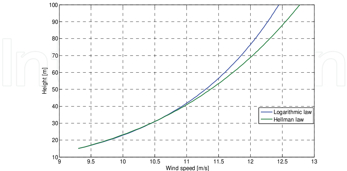
Fig. 2. Wind profile built up using the logarithmic law and the Hellman law applicable to rural areas
