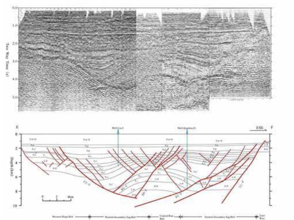
Fig. 8. Qiaokou section of the middle of the Dongpu Sag (see E-F in Fig. 1 for location). CY-F: Changyuan fault, HH-F: Huanghe fault, DZ-F: Duzhai fault, LL-F: Lanliao fault, WX-F: Wenxi fault. Lanliao fault soles out in the detachment surface of 14-16 km deep
