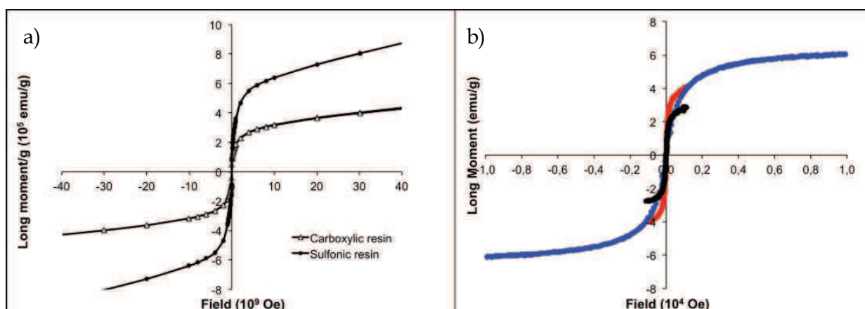
Fig. 10. a) SQUID hysteresis curves of \text{Pd@Co} NPs in carboxylic and sulfonic resins and, b) SQUID hysteresis curve of ferrite core NPs synthesized in sulfonic resin: blue) \text{Ag@Fe}_3\text{O}_4 , red) \text{Fe}_3\text{O}_4 , black) \text{Ag@Fe}_3\text{O}_4 half concentration compared with blue).
