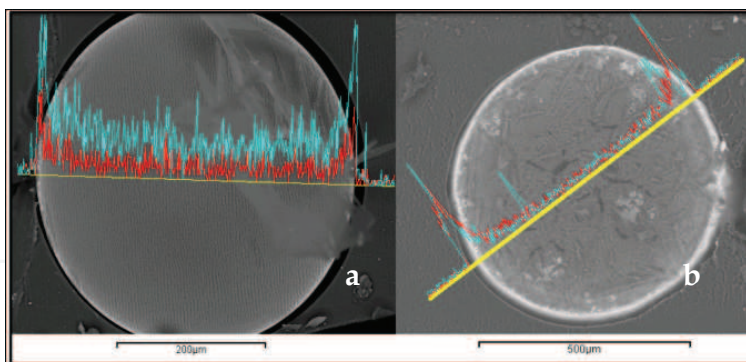
Fig. 9. SEM images of ferric oxide NPs in sulfonic ion exchange polymers: a) \text{MnFe}_2\text{O}_4 gel-type resin where the blue line represents Mn and the red line represents Fe, and b) \text{Ag@Fe}_3\text{O}_4 gel-type resin where blue line represents Ag and the red line represents Fe.
