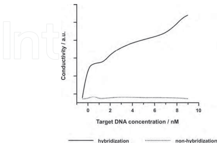
Fig. 2. The curve of the DNA sequence hybridization.
