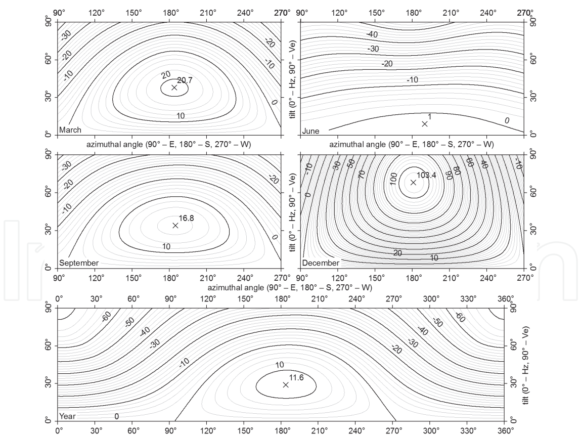
Fig. 6. Contour plots of the relative PV array energy yield regarding the horizontal surface as a function of a fixed orientation and tilt for March, June, September and December as well as the whole year for Portorož in the Mediterranean part of Slovenia.
