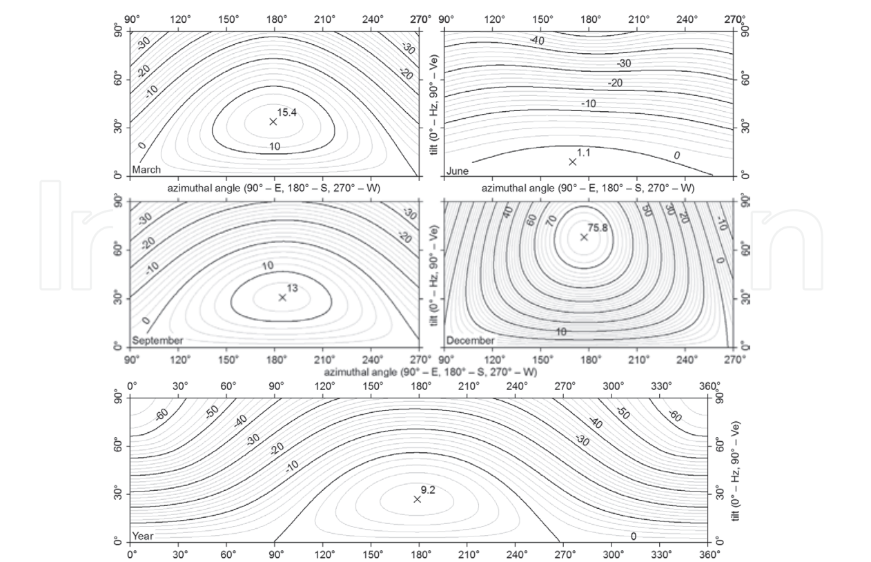
Fig. 9. As for Figure 6, but for Murska Sobota in the Pannonian part of Slovenia
