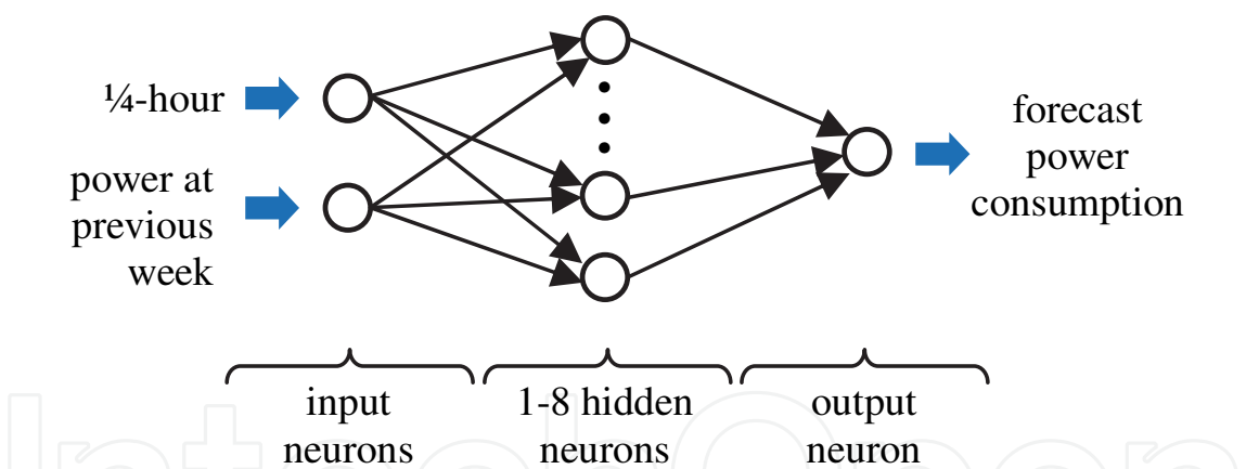
Fig. 11. Network for the power demand
