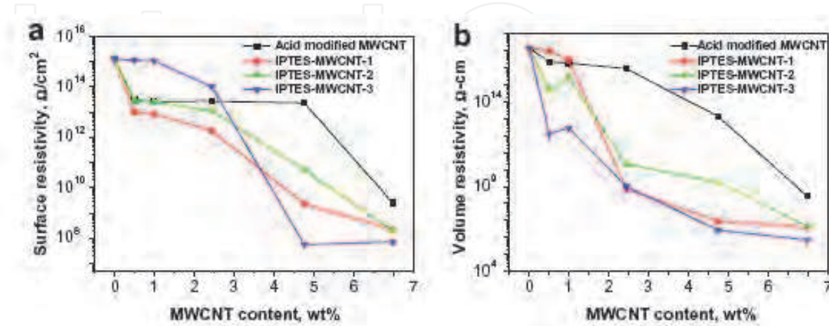
Fig. 15. Electrical behavior of acid and IPTES modified MWNTs poyimide nanocomposites, a) Surface resistivity, b) Volume resistivity. Copyright Elsevier Science
