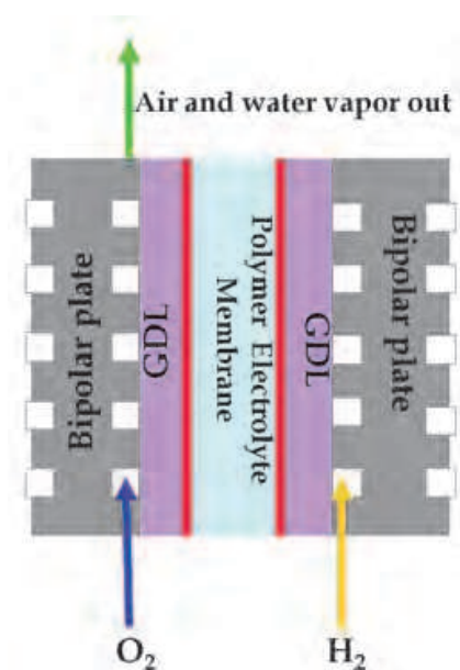
Fig. 1. Exploded view of PEMFC components
