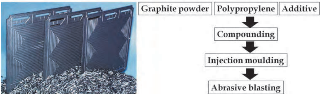
Fig. 18. ©Sigracet PPG86 bipolar plates and their production [52]
