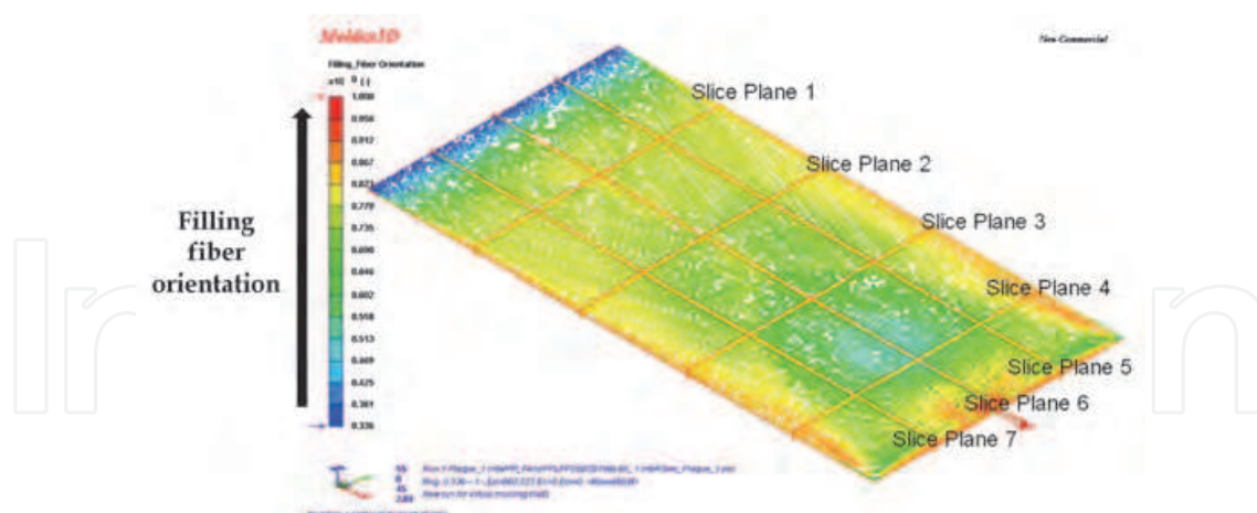
Fig. 22. Simulation output fibre orientation-skin [11]
