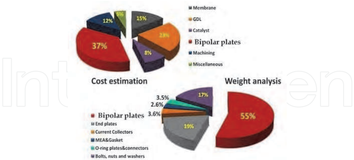
Fig. 3. Relative cost and weight components from a PEMFC using graphite bipolar plate [11]
