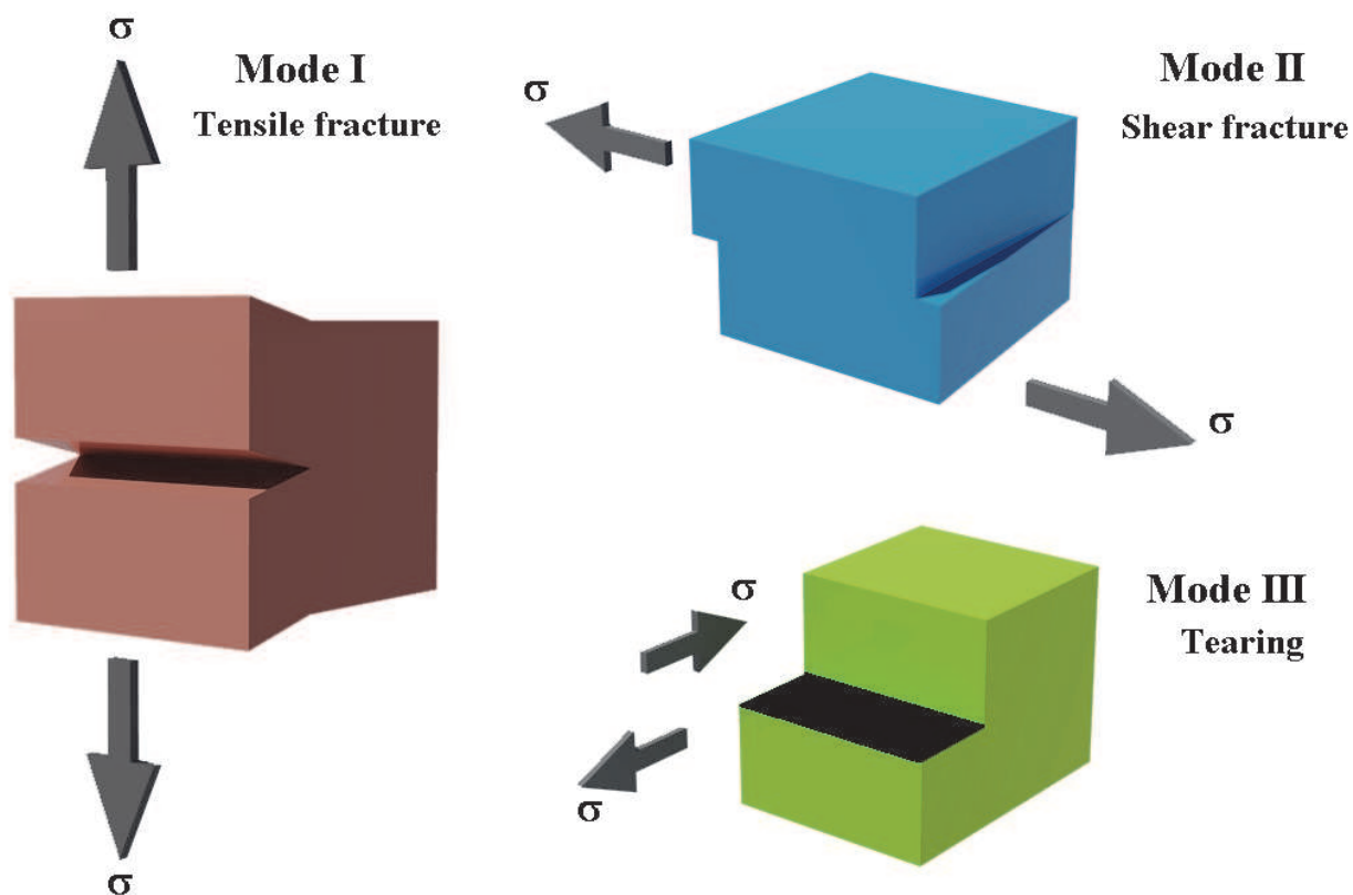
Fig. 6. Fracture modes.
