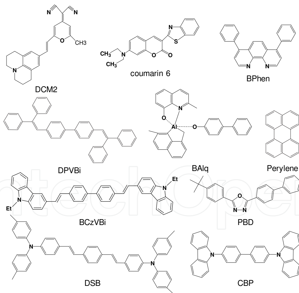
Fig. 11. Molecular structures of used organic materials.
