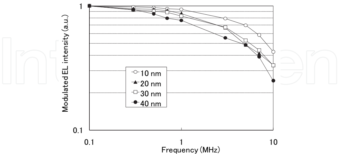
Fig. 7. Relative EL intensity while applying the sine wave voltage for OLEDs with different thicknesses of the ETLs. (Fukuda et al., 2007e)
