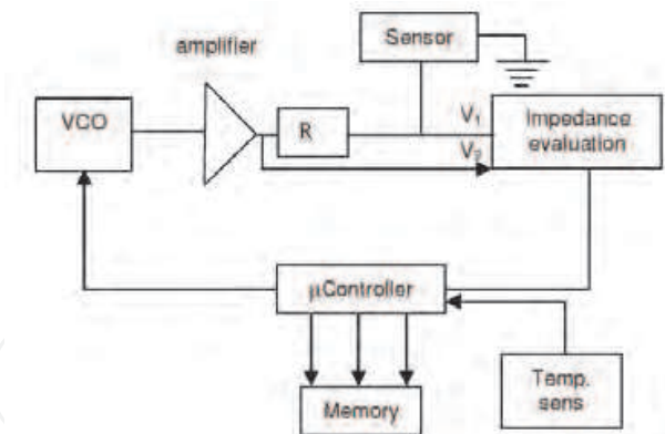
Fig. 7. Block diagram of the impedance spectroscopy based blood glucose sensor
