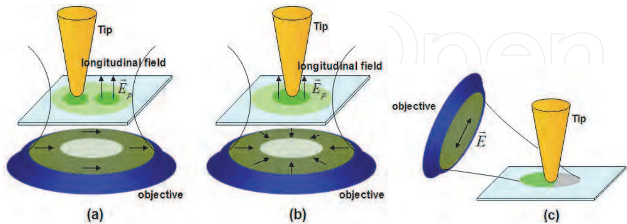
Fig. 3. Schematic diagrams of tip-enhanced Raman spectroscopy using (a) linearly polarized light (or beam) annular illumination; (b) radially polarized annular illumination; (c) linearly polarized side illumination.
