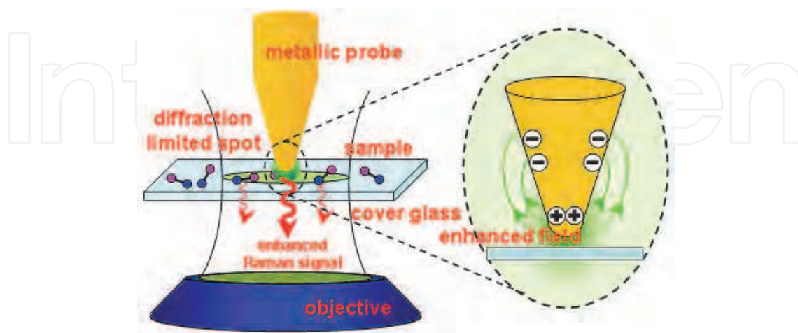
Fig. 1. Concept of tip-enhanced Raman spectroscopy (TERS) shows a strongly enhanced optical field generated at the apex of sharp metal tip of SPM by the external illumination (R. Wang, 2010c).
