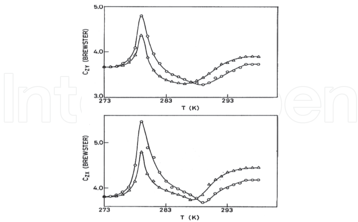
Fig. 16. Anomalous temperature dependence of the piezo-optic coefficients C_{zx} and C_{zy} of the crystals LGO in a cooling (○) and heating (Δ) cycle.
