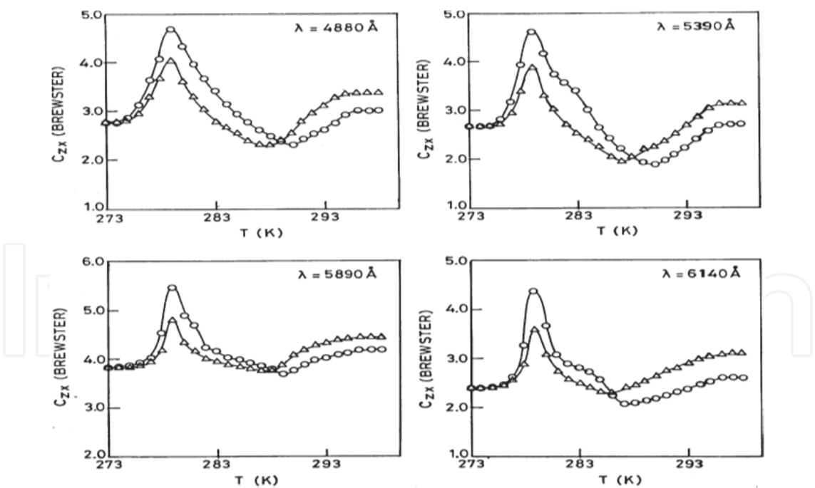
Fig. 17. Anomalous temperature dependence of piezo-optic coefficient C_{zx} of the crystals LGO at different wave lengths in a cooling (○) and heating (Δ) cycle.
