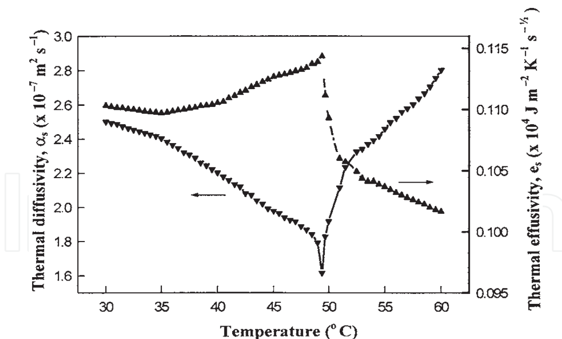
Fig. 4. (a) Variations of the thermal diffusivity (inverted triangles) and thermal effusivity (triangles) with temperature for TGS along the b axis (Menon & Philip, 2000)
