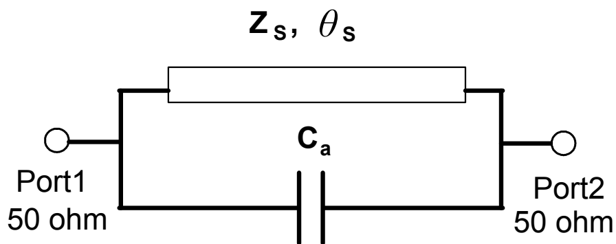
Fig. 5. Schematic of the lowpass filter.
