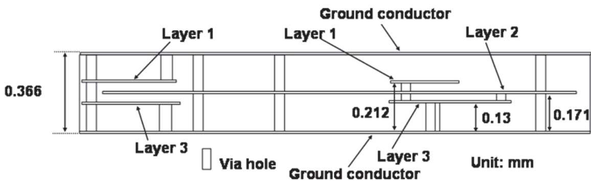
Fig. 11. Cross sectional structure of the filter.
