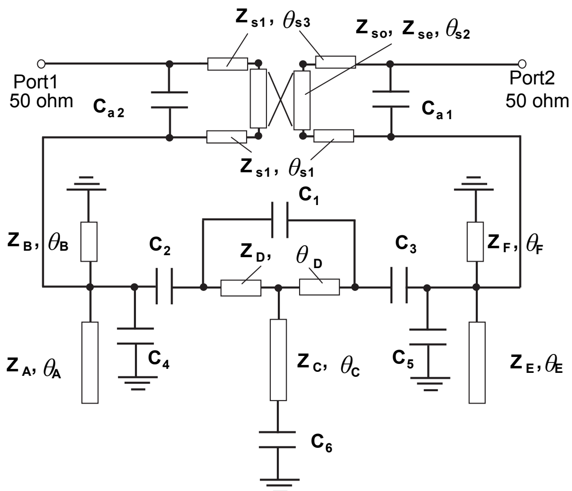
Fig. 7. Schematic of the bandpass filter.
