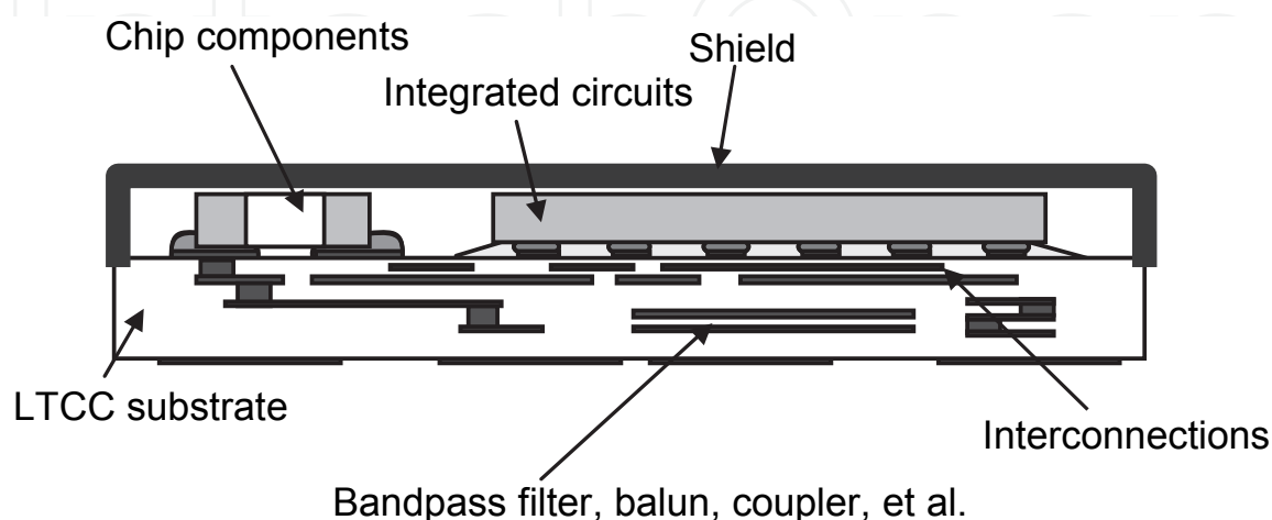
Fig. 1. A general structure of the compact wireless module using the LTCC technology.
