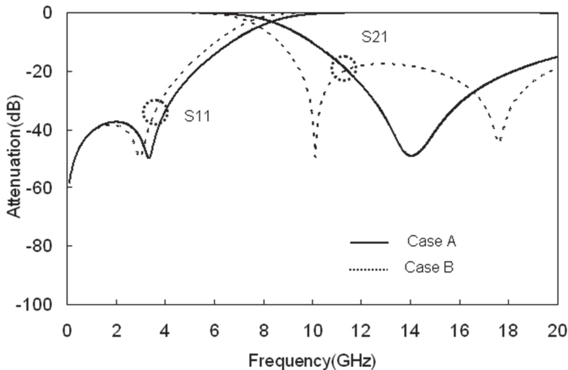
Fig. 6. Simulated results of the lowpass filter shown in Fig.5.
