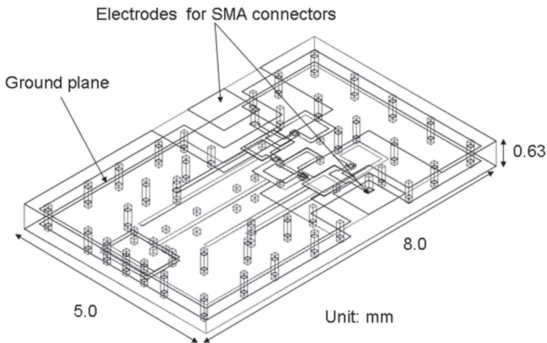
Fig. 14. Structure of the LTCC substrate for evaluation.
