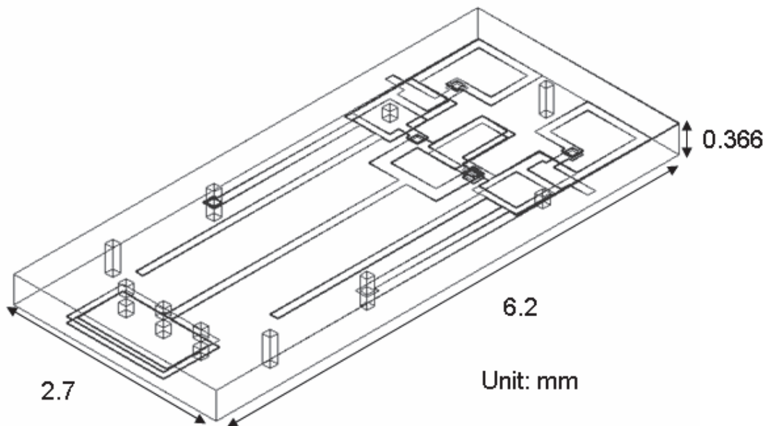
Fig. 10. Three-dimensional structure of the filter.
