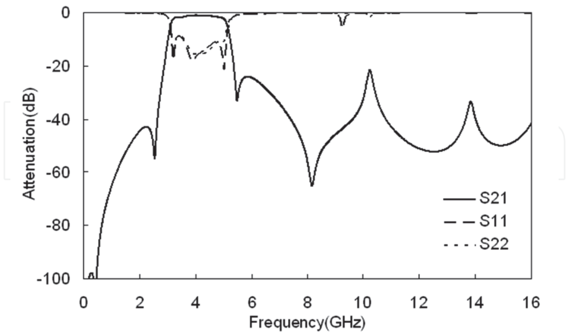
Fig. 13. Simulated results by the electromagnetic simulator.
