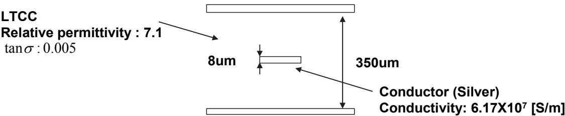
Fig. 3. Physical model for a stripline.
