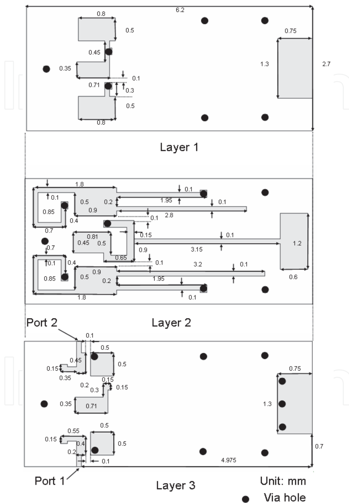
Fig. 12. Top view of the filter.
