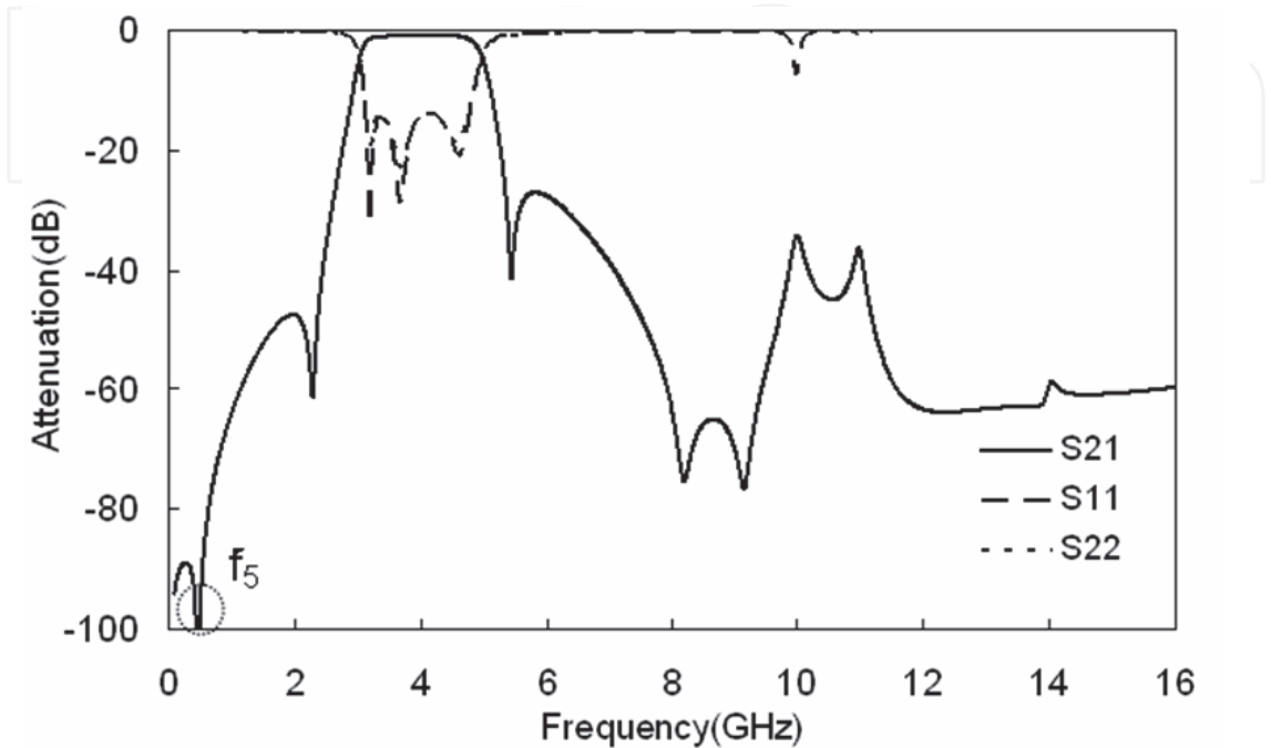
Fig. 8. Simulated results of the filter shown in Fig.7.
