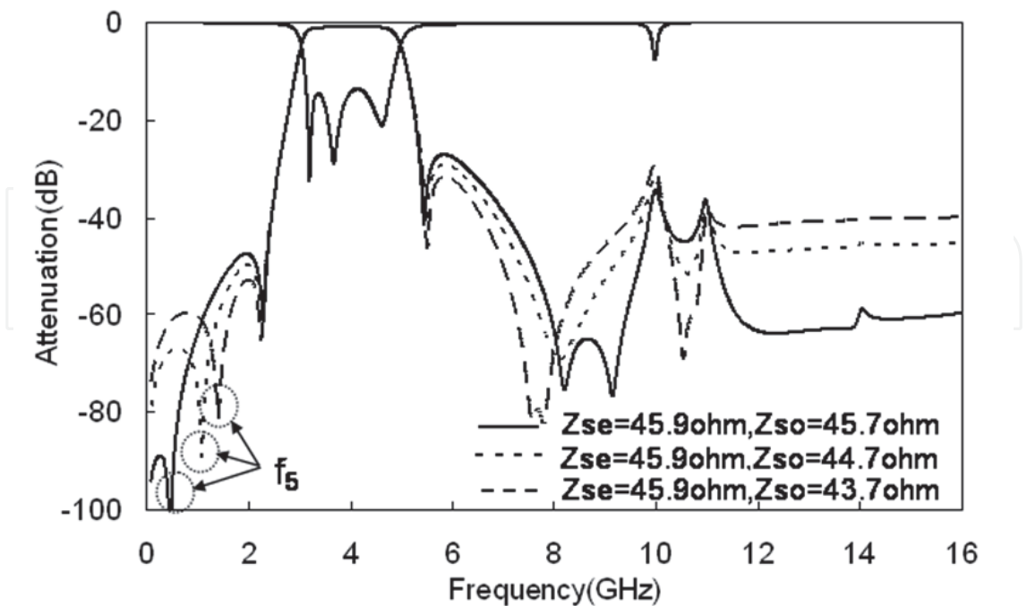
Fig. 9. Simulated results of the filter shown in Fig.7, when the coupling condition of the stripline is varied.
