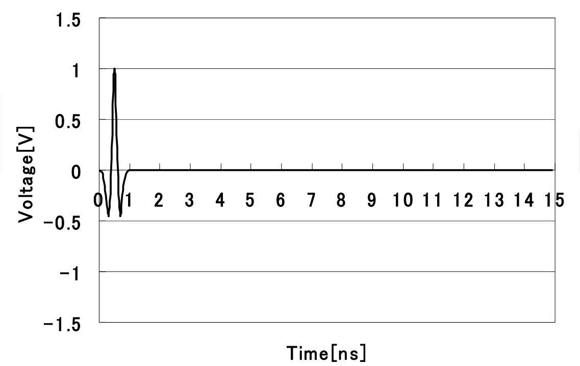
(1) 1 pulse sequence under the CM1 environment
