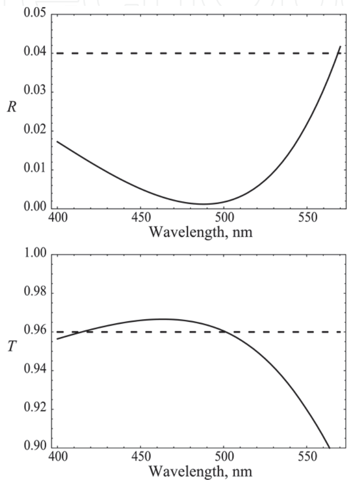
Fig. 7. Reflectance R and transmittance T of a composite slab with silver nanoparticles for normal incidence of light, calculated within the effective-medium model. The reflectance and transmittance of the clean dielectric surface are shown for comparison by dashed lines.
