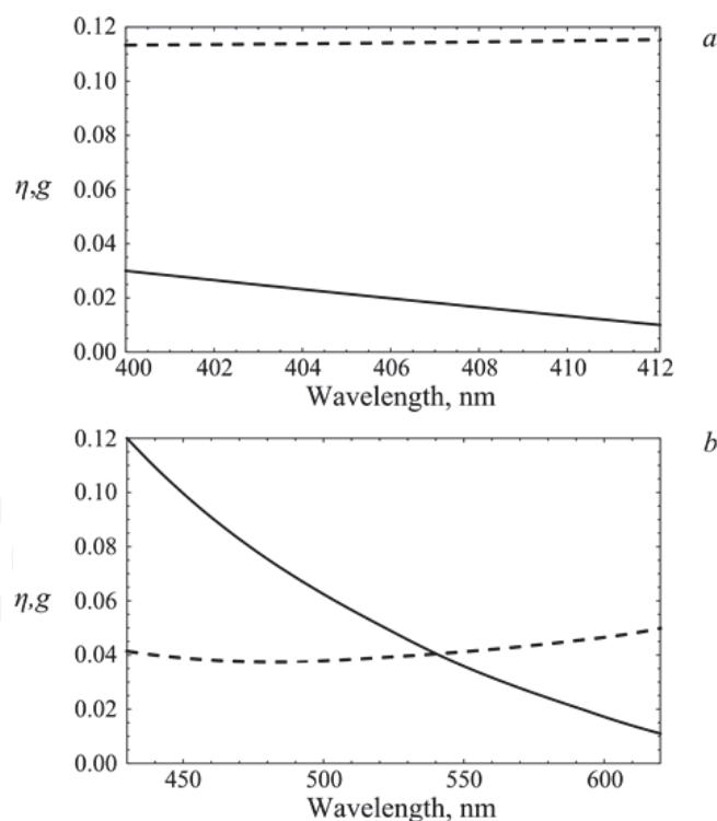
Fig. 5. Gain g of matrix ( dashed lines ) and the volume concentration \eta ( solid lines ) of spherical (a) and needle-like (b) nanoparticles are required to produce a transparent composite material with the unit index of refraction. The radius of the spherical particle is equal to 7 nm, the volume of the spheroid with \xi = 3 is equal to that of a spherical particle. The external field is oriented parallel to the spheroid revolution.
