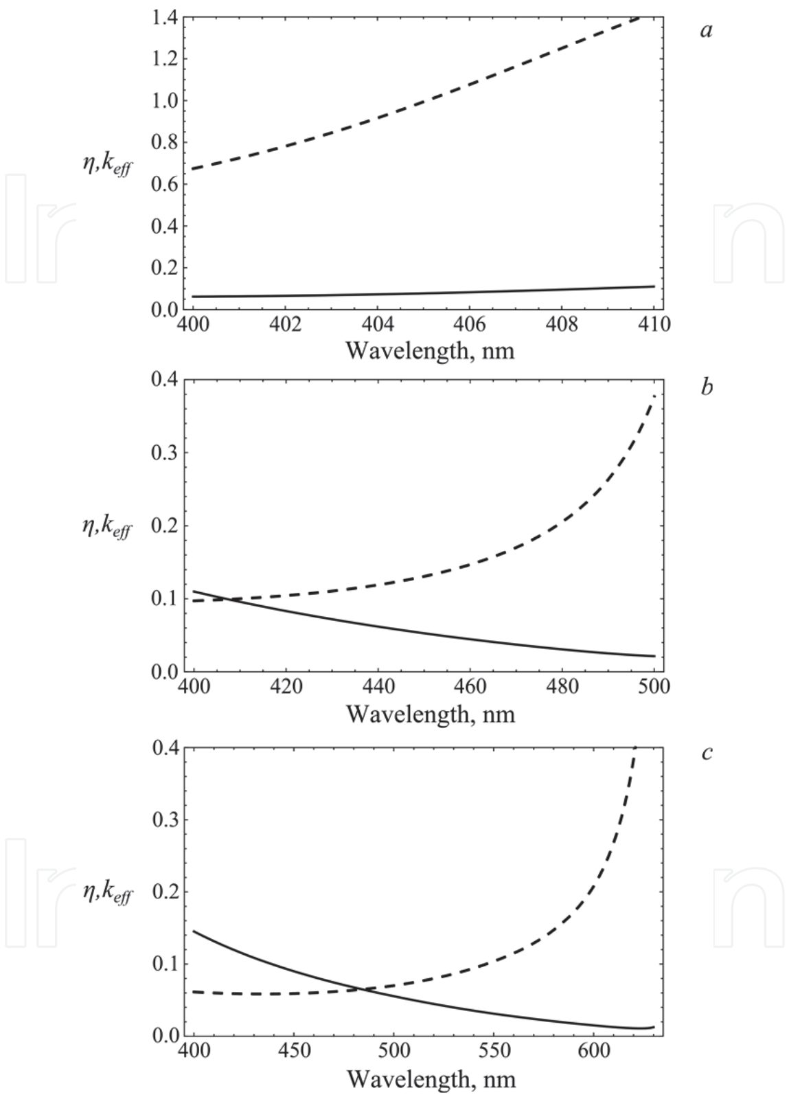
Fig. 4. Effective extinction coefficient k_{eff} (dashed lines) and the volume fraction of inclusions \eta (solid lines) of a composite medium with the unit effective refractive index. Silver inclusions are spherical particles (a) and flattened (b) and elongated (c) spheroids. Particle parameters are the same as given in Fig. 3.
