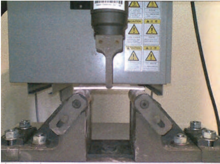
Fig. 10. Three point bending test setup
