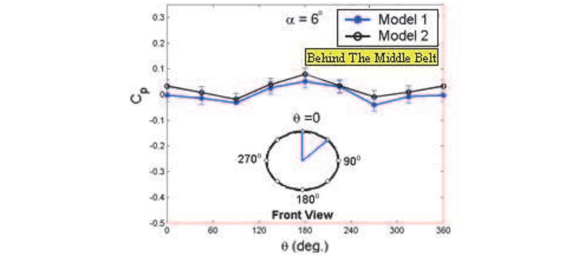
b) Circumferential pressure distributions behind the middle belt ( x/d=11.25 ).
