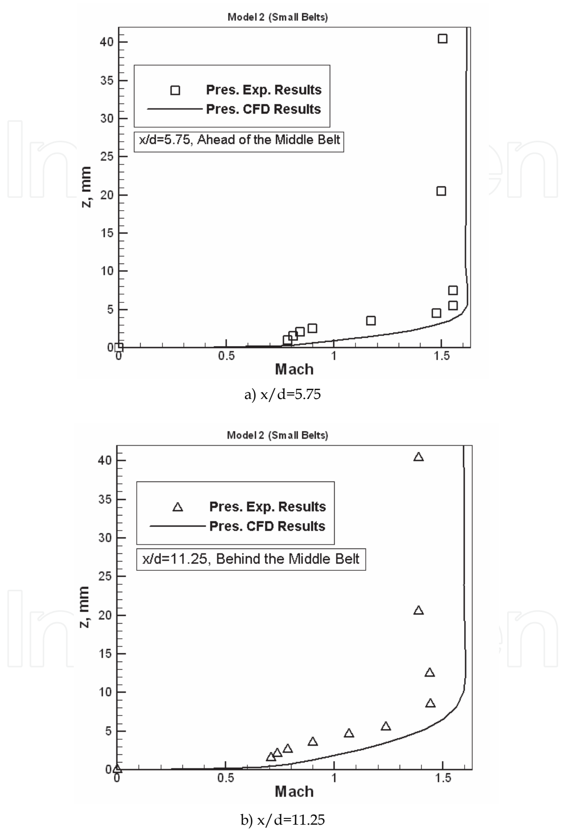
Fig. 11. Experimental and numerical boundary layer profiles for model 2 at \alpha = 0 .
