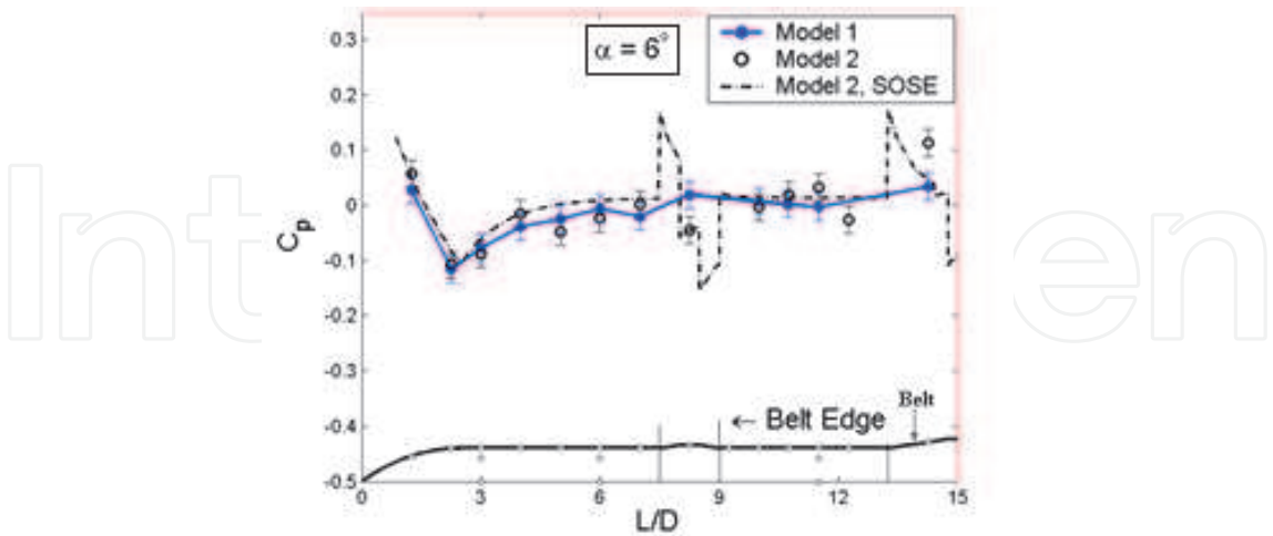
a) Experimental, theoretical, and numerical longitudinal pressure distribution.
