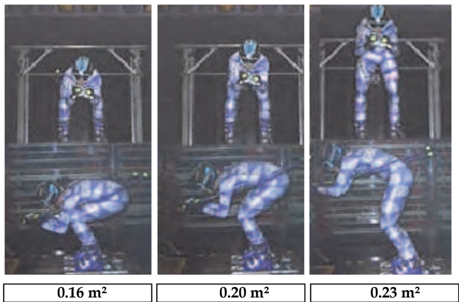
Fig. 4. Variation of the A.C_D factor of a downhill skier according to posture variations (Wind tunnel of IAT, France).
