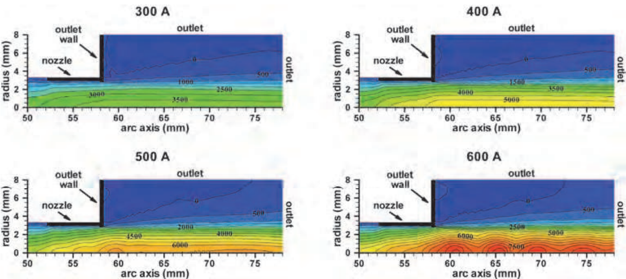
Fig. 10. Velocity contours in the outlet nozzle and near-discharge regions for 32 slm of argon. Partial characteristics radiation model is employed. Water mass flow rates are 0.228 g · s -1 (300 A), 0.315 g · s -1 (400 A), 0.329 g · s -1 (500 A), 0.363 g · s -1 (600 A), contour increments are 500 m · s -1 . Supersonic flow structure is obvious for 600 A.
