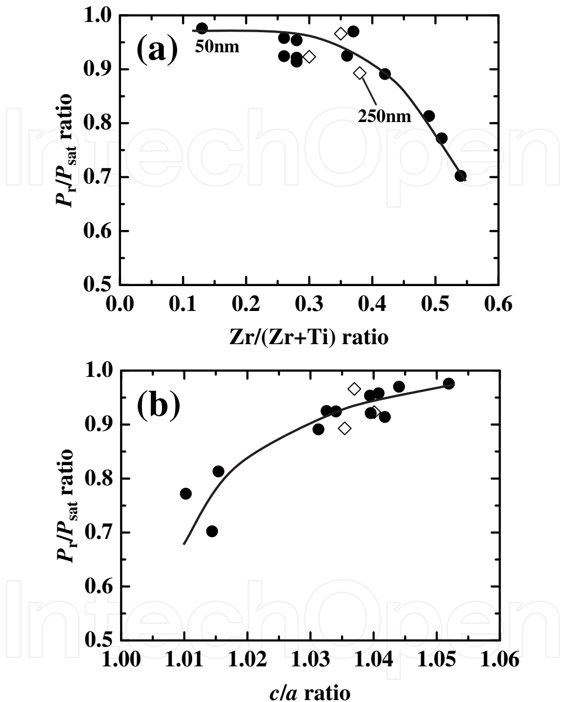
Fig. 15. Evolution of P_r/P_{sat} ratio as function of Zr/(Zr+Ti) ratio (a) and c/a ratio (b)
