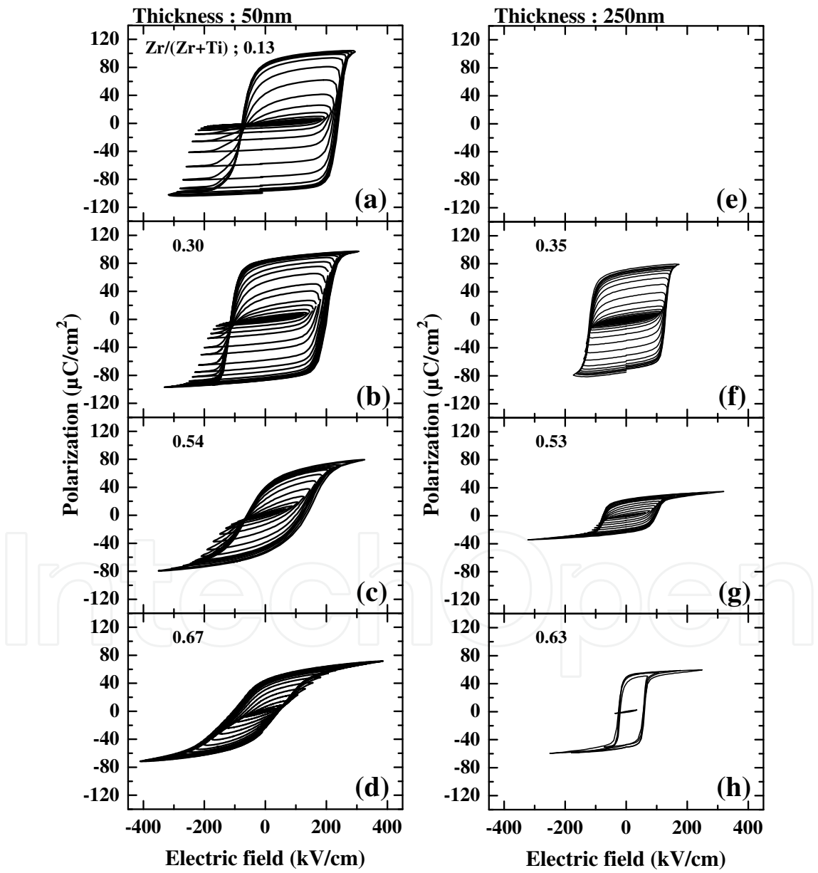
Fig. 10 Polarization - electric field ( P - E ) relationships for films with various Zr/(Zr+Ti) ratio and film thickness. from 50 nm thick films [(a)-(d)] and 250 nm thick films [(e) - (h)].
