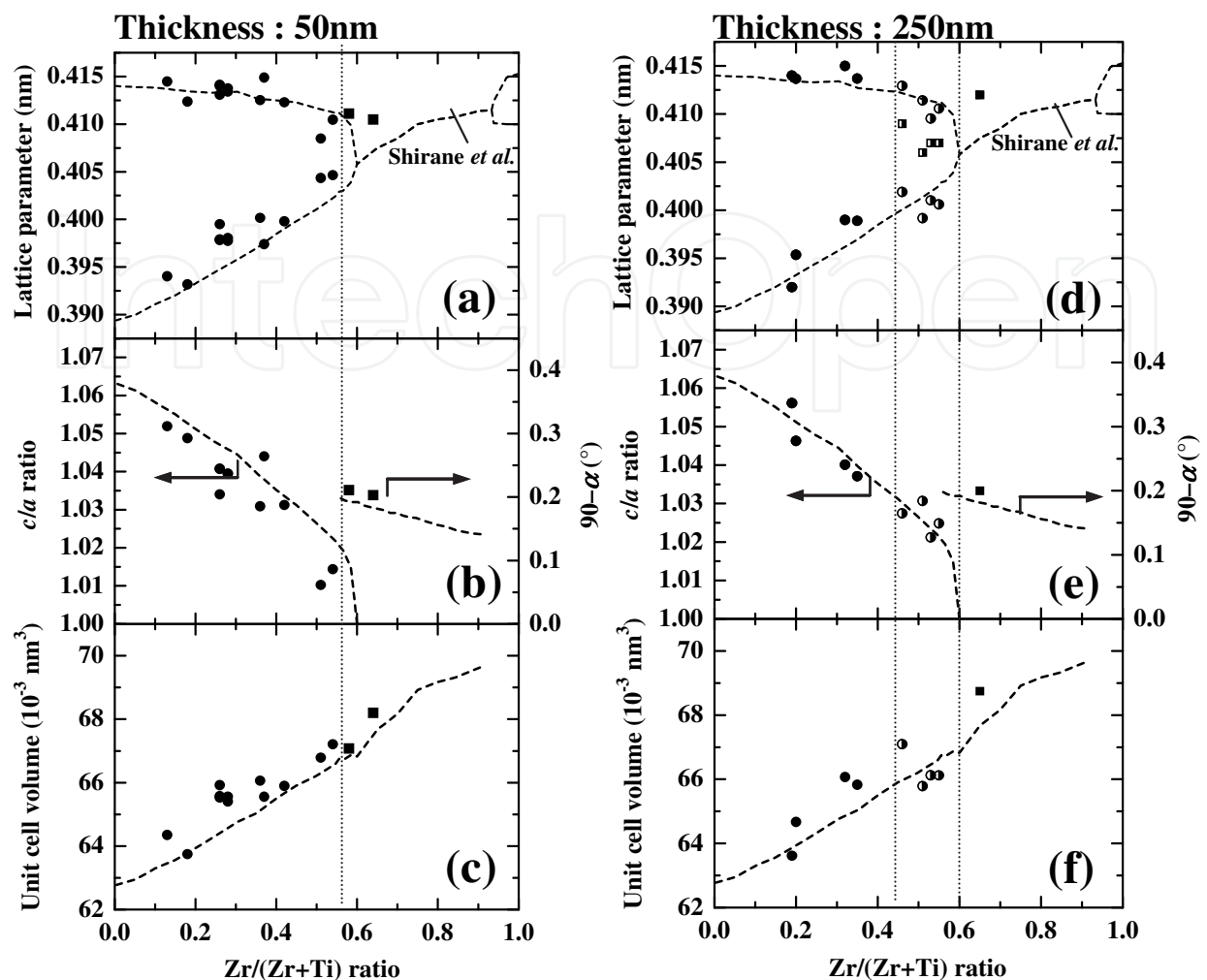
Fig. 7. Lattice parameters (a, d), tetragonality, c/a ratio, and the internal angles and (b, e), and unit cell volume (c, f) as a function of \text{Zr}/(\text{Zr}+\text{Ti}) ratio for (a)-(c) 50 and (d)-(f) 250 nm thick films. Dashed lines are powder data reported by Shirane et al (Shirane & Suzuki, 1952).
