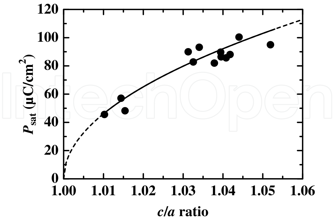
Fig. 13. Relationship between P_{sat} and the c/a ratio of PZT films.
