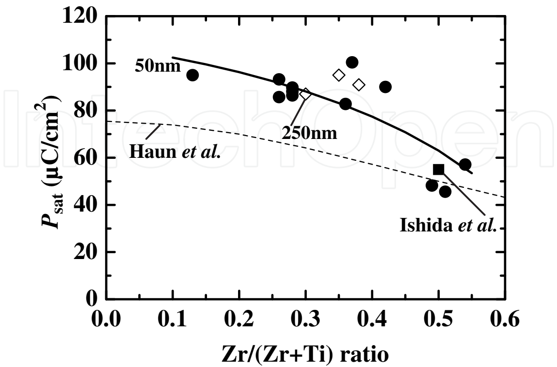
Fig. 12. Estimated P_{sat} as a function of Zr/(Zr+Ti) ratio in films.
