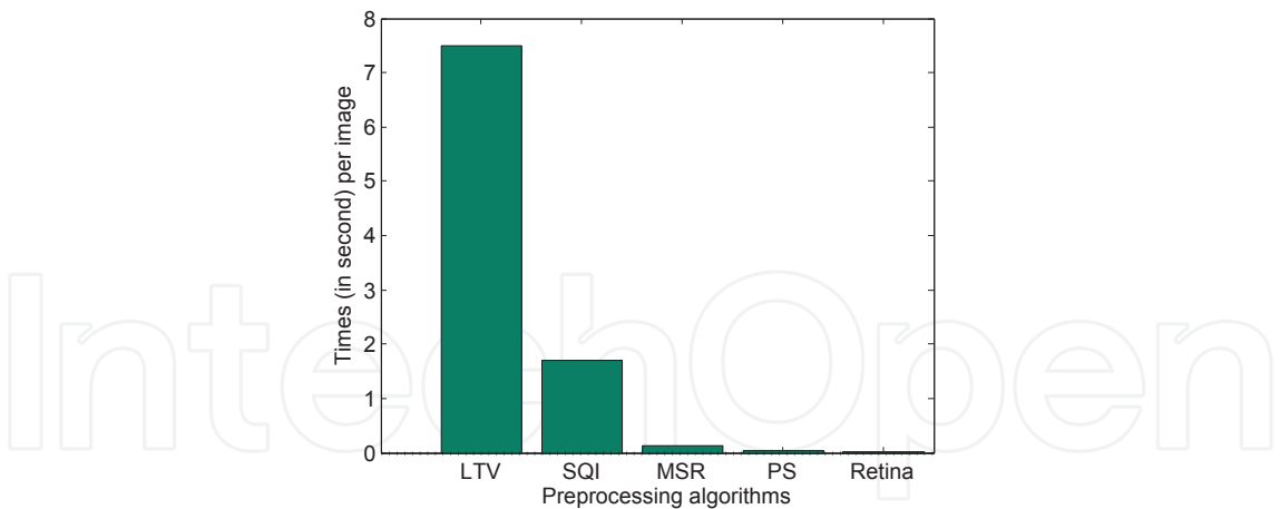
Fig. 16. Average computational time of different algorithms on a 192 \times 168 image.
