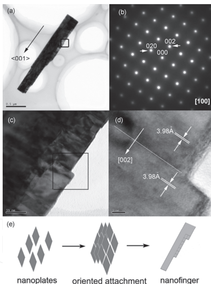
Fig. 7. The TEM results and the formation mechanism of a single K_{0.5}Na_{0.5}NbO_3 nanofinger. (a) TEM image; (b) SAED patterns; (c) magnified image of the marked area in (a); (d) HRTEM image of the marked area in (c).
