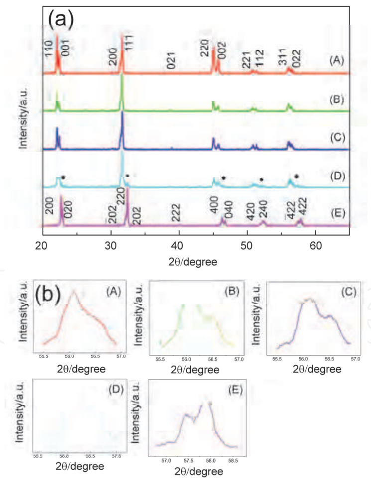
Fig. 4. (a) The XRD patterns in the 2\theta range of 20^\circ to 65^\circ of the as-synthesized K_{1-x}Na_xNbO_3 materials with different compositions; (b) The enlarged XRD patterns in the 2\theta range of 55^\circ to 58^\circ , which suggest the phase transition by the symmetry changes of the diffraction peaks.
