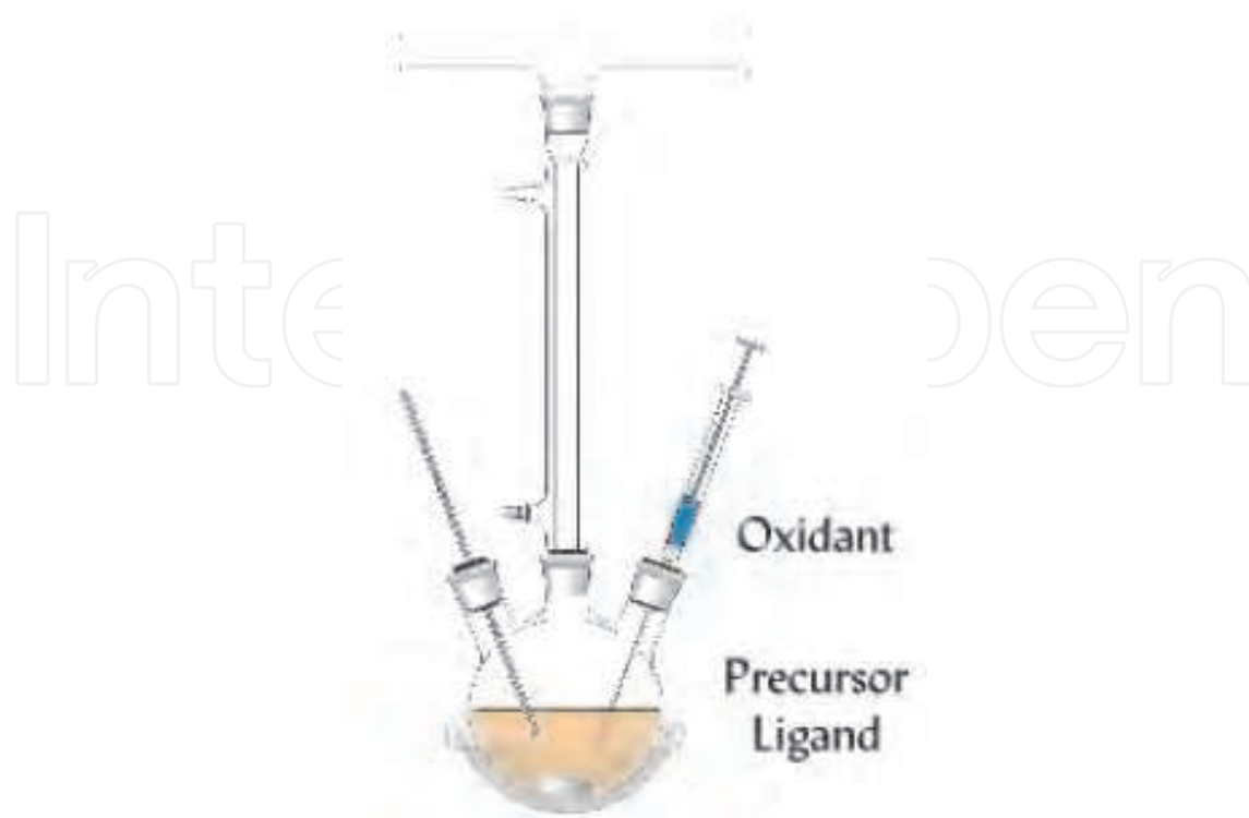
Fig. 1. A schematic illustration of a typical solution-phase decomposition (taken from reference 4).
