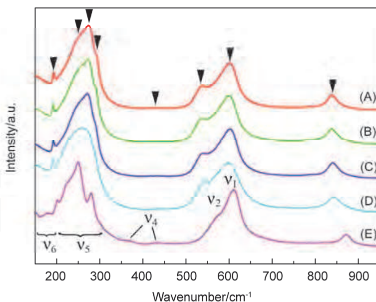
Fig. 8. The room-temperature Raman scattering spectra of the as-synthesized \text{K}_{1-x}\text{Na}_x\text{NbO}_3 with different compositions derived from a hydrothermal method.
