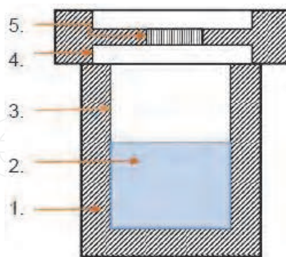
Fig. 2. A schematic illustration of a typical autoclave used in hydrothermal method, which is consist of (1) stainless steel autoclave (2) precursor solution (3) Teflon liner (4) stainless steel lid and (5) spring.
