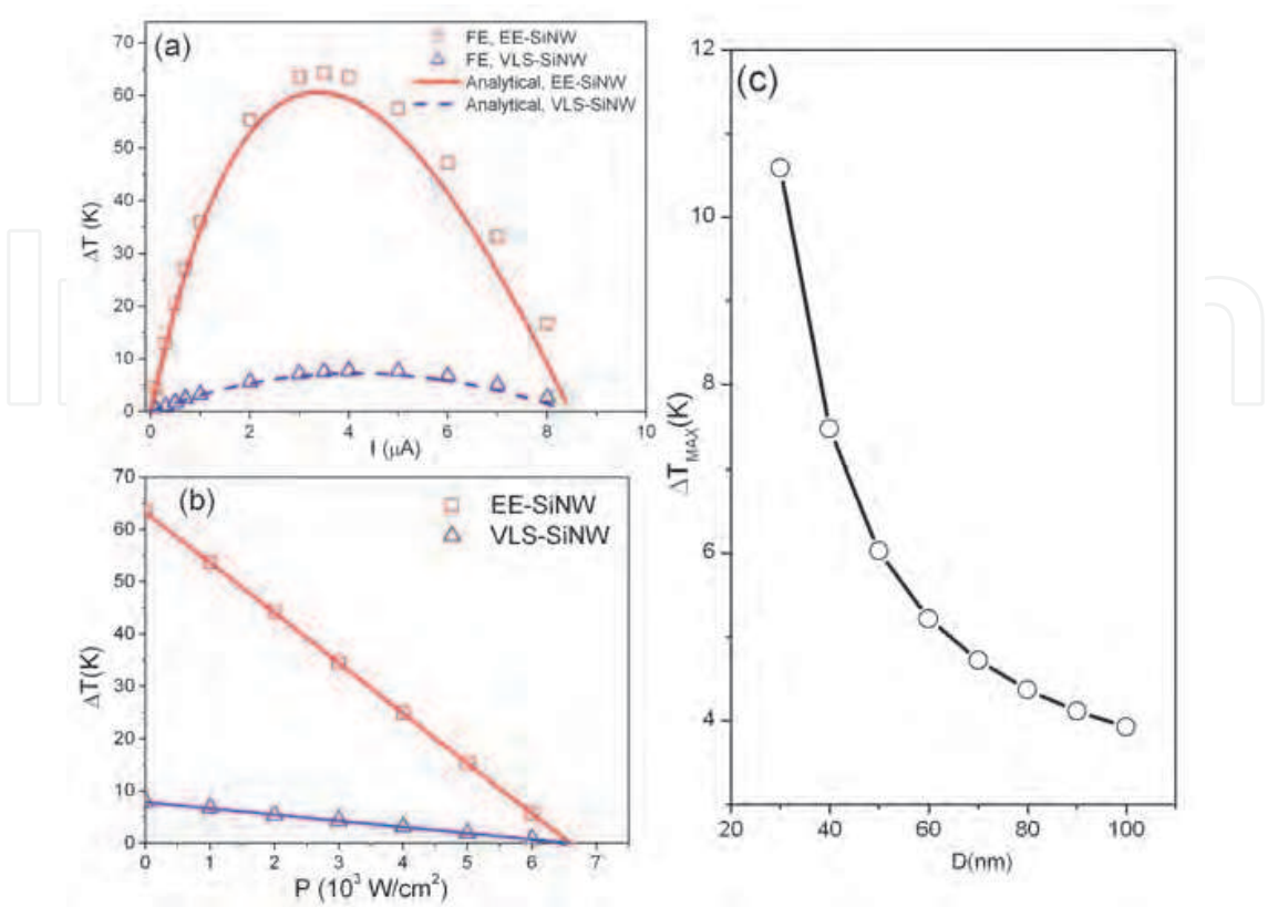
Fig. 11. (a) Dependences of cooling temperature on thermal conductivity and applied electrical current. (b) Cooling temperature versus heat load power density. (c) Maximum cooling temperature vs diameter of SiNW.
