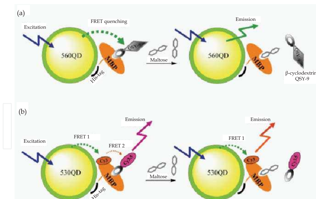
Fig. 6. QD based maltose nanosensor. (a) \beta -CD-QSY-9/MBP complex bound to QD through a peptide His-tag; (b) \beta -CD-Cy3.5/MBP-Cy3 complex bound to QD through a peptide His-tag (Zhou, 2007).
