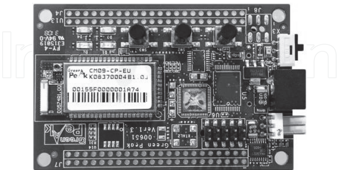
Fig. 3. WSN sensor node with integrated temperature sensor (Power provided by 3 AAA bateries placed underneath)
