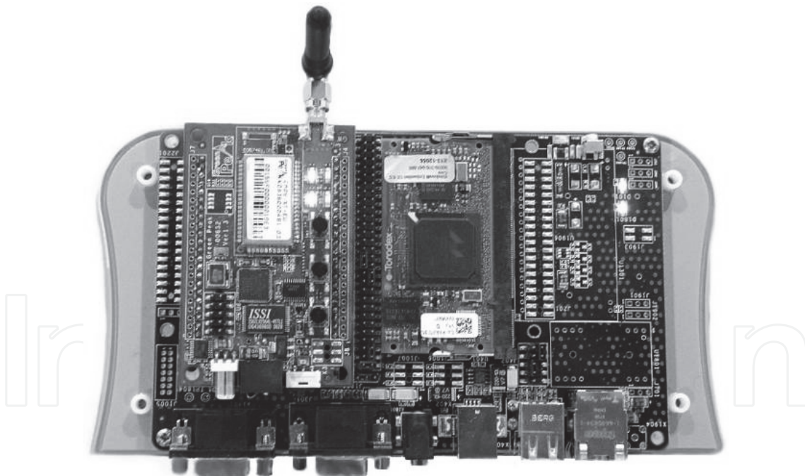
Fig. 4. Gateway/Coordinator node built around a RISC microcontroller
