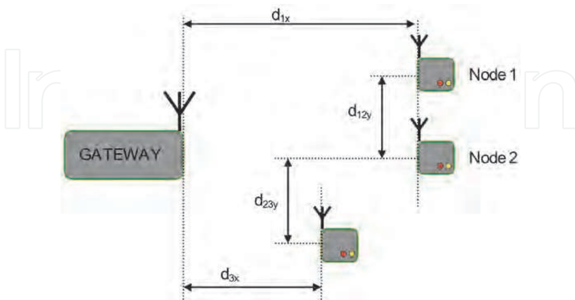
Fig. 7. Test setup with the Gateway and three WSN nodes ( d_{1x}=2.5\text{m} , d_{3x}=2.2\text{m} , d_{12y}=0.4\text{m} , d_{23y}=0.8\text{m} )
