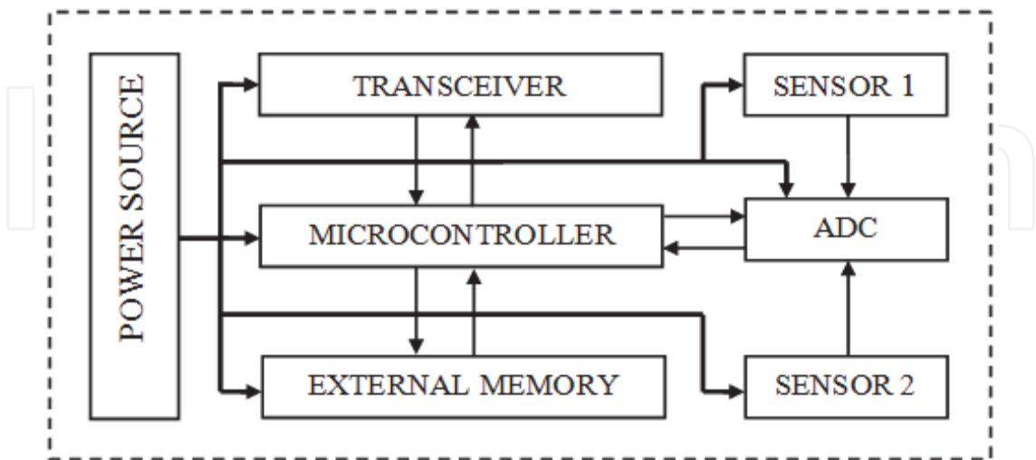
Fig. 2. WSN node architecture
