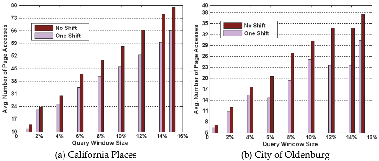
Fig. 9. Comparison on shift.
