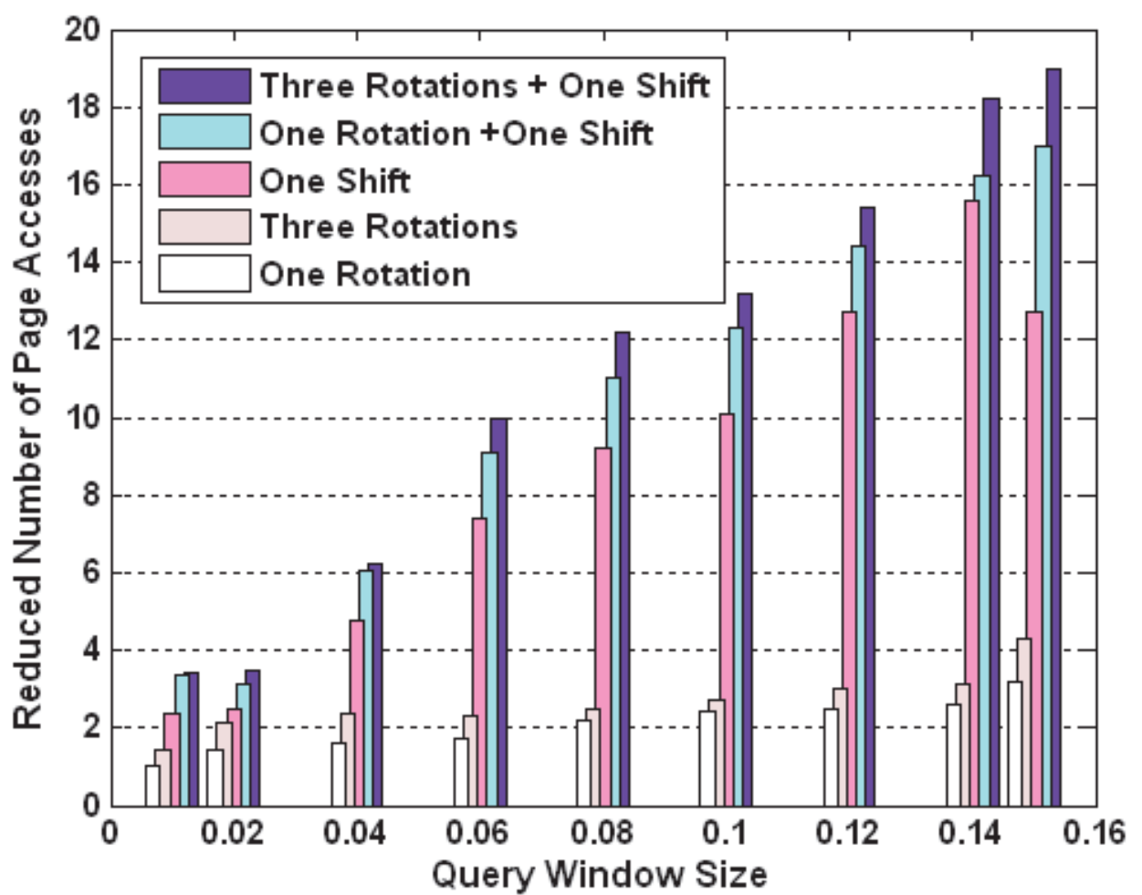
Fig. 10. Efficiency comparisons.
