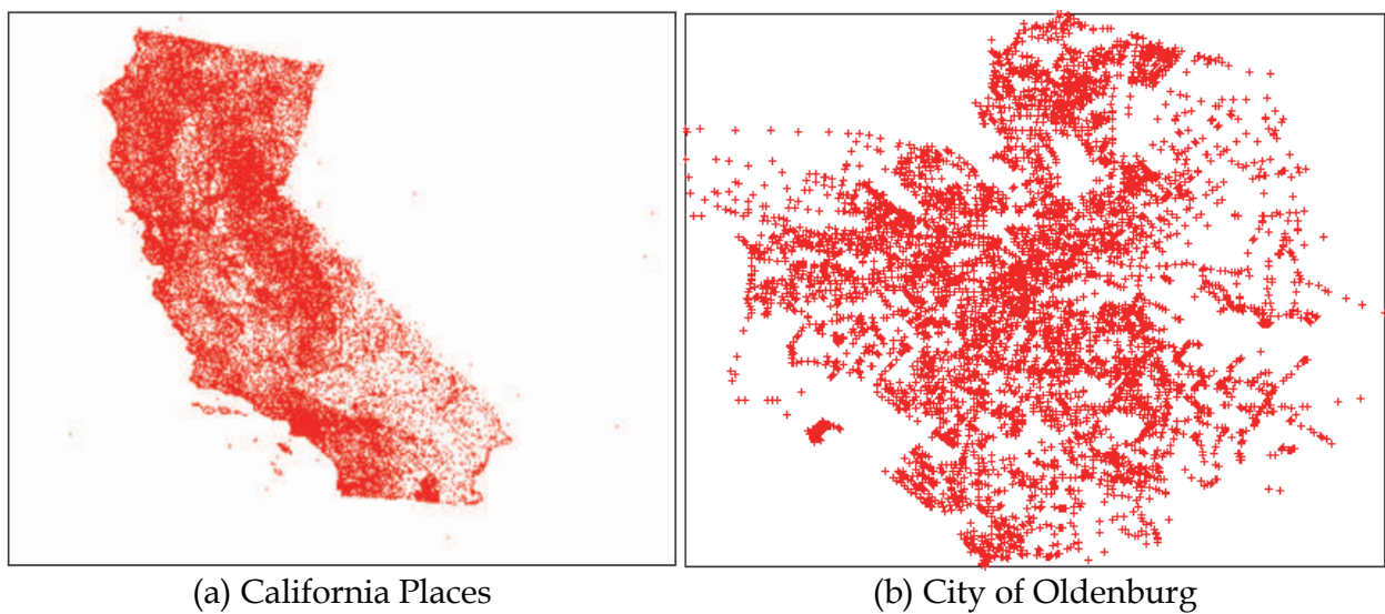
Fig. 6. Datasets.
