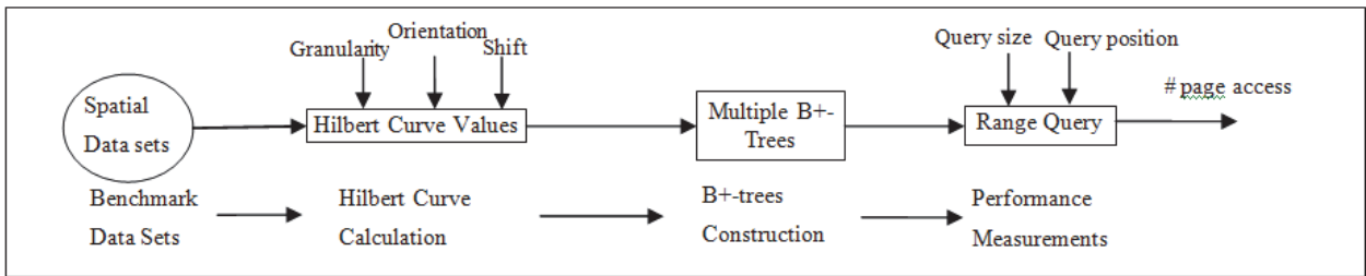
Fig. 7. Experimental design.
