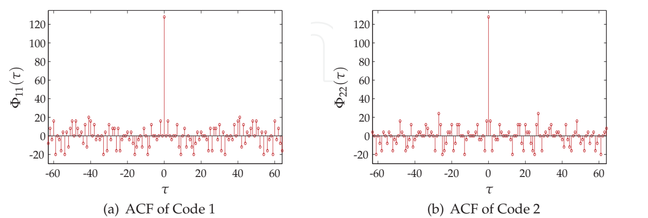
Fig. 14. ACF of adjusted Gold codes
