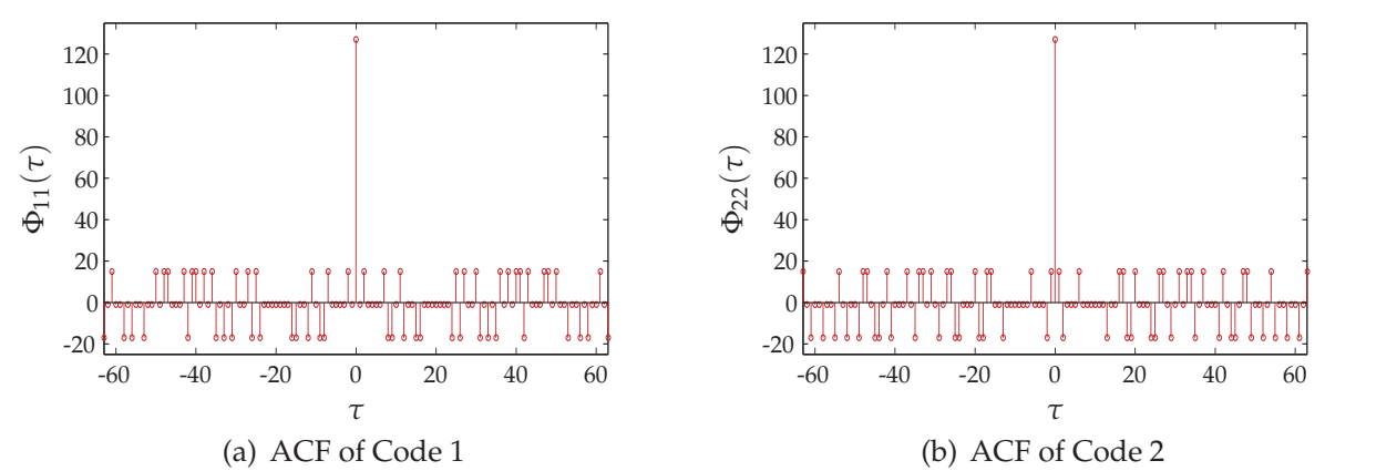
Fig. 13. ACF of original Gold codes
