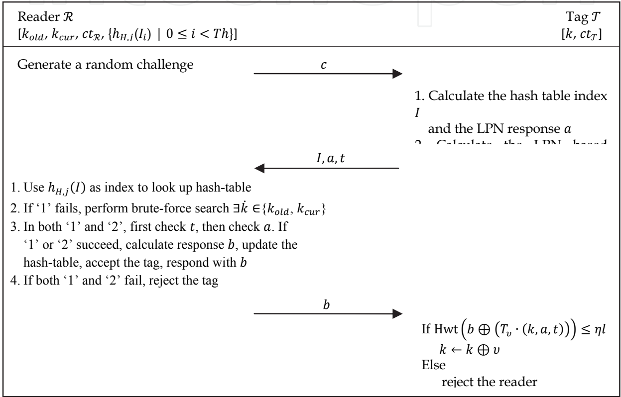
Fig. 3. The Proposed F-HB + Protocol
