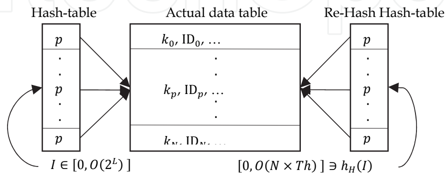
Fig. 1. The traditional Hash-table vs. basic Re-Hash hash-table
