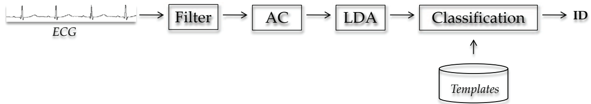
Fig. 3. Block diagram of the AC/LDA algorithm.
