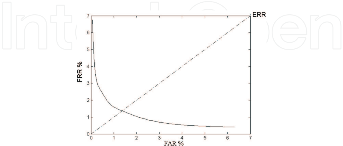
Fig. 17. ROC curve of the method
