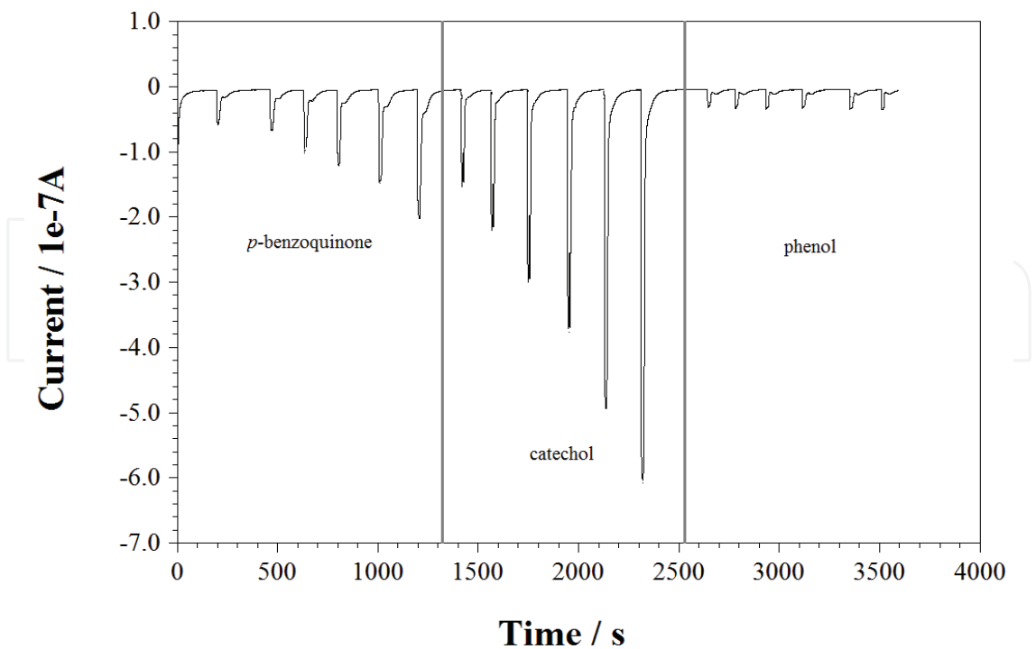
Fig. 5. Poly(GA-co-Py)/HRP composite film electrode response to 75-125-200-300-500-750 \mu M p -benzoquinone, catechol and phenol injections. Applied potential was -50 mV (vs. Ag/AgCl, 3 M NaCl).
