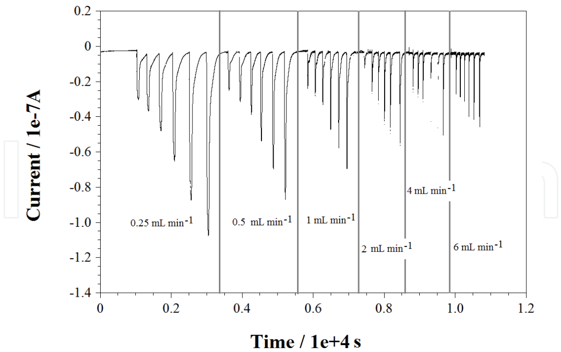
Fig. 6. Effect of 0.25-0.5-1-2-4-6 mL min -1 flow rate on Poly(GA-co-Py)/HRP composite film electrode response to 75-125-200-300-500-750 \mu M p -benzoquinone injections. Applied potential was -50 mV (vs. Ag/AgCl, 3 M NaCl).
