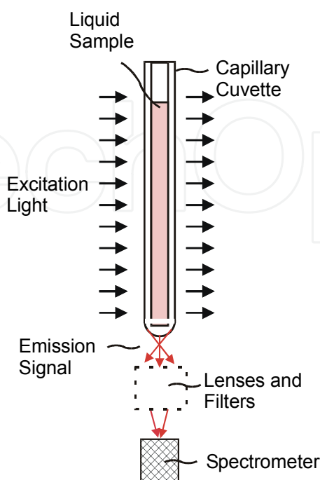
Fig. 1. Integrating Waveguide Technology detection concept.
