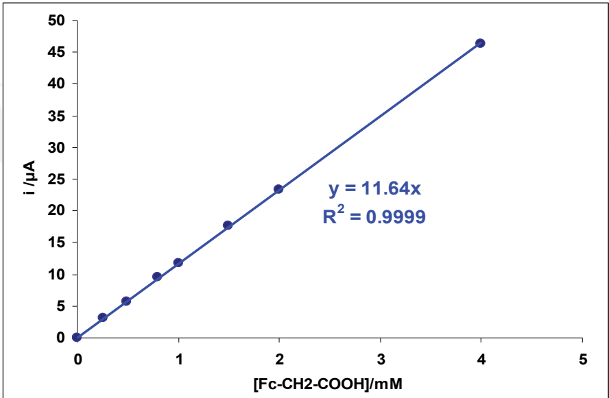
Fig. 6. Calibration curve of carboxymethyl ferrocene
