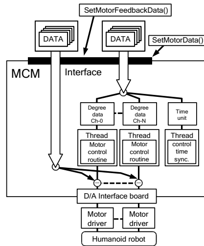
Figure 8. The model of Motor Control Module (MCM)
