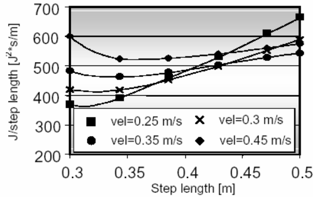
Figure 21. CE vs. the walking velocity
