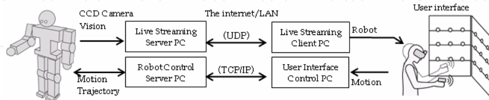
Figure 27. Schema of humanoid robot teleoperation system
