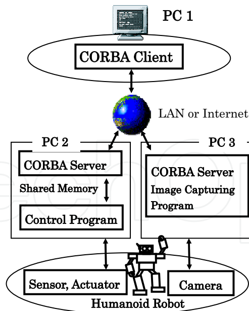
Figure 39. Teleoperation concept
