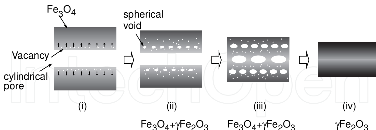
Fig. 9. Schematic illustrations of transition in the morphology of a \text{Fe}_3\text{O}_4 nanotube: (i) dissociation and outward diffusion of vacancies at the inner surface of a nanotube of \text{Fe}_3\text{O}_4 , (ii) formation of additional spherical voids associated with shrinkage of an interior pore and phase transformation from \text{Fe}_3\text{O}_4 to \gamma\text{-Fe}_2\text{O}_3 , (iii) growth of voids and shrinkage of an interior pore, and (iv) the formation of nonporous \gamma\text{-Fe}_2\text{O}_3 . Vacancies are generated from inner surface and diffuse outward. The outward vacancy diffusion accompanies the phase transformation from \text{Fe}_3\text{O}_4 to \gamma\text{-Fe}_2\text{O}_3 . The vacancies combine to form voids during the diffusion process. (Reproduced with permission from the reference (Nakamura et al, 2009a))
