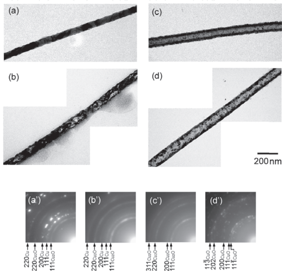
Fig. 4. BFIs of Cu nanowires (a) before oxidation and after oxidation (b) at 423 K for 1.2 ks, (c) at 423 K for 5.4 ks and (d) at 573 K for 3.6 ks and their corresponding SAED patterns (a' - d'). (Reproduced with permission from the reference (Nakamura et al, 2009b))
