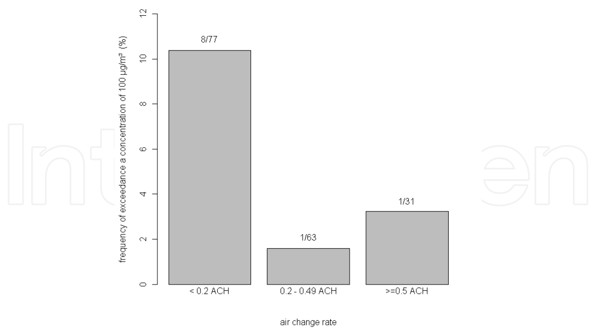
Fig. 16. Frequency of formaldehyde concentrations >100 µg/m³ and ACR (natural ventilation) in rooms of the City of Berlin.
