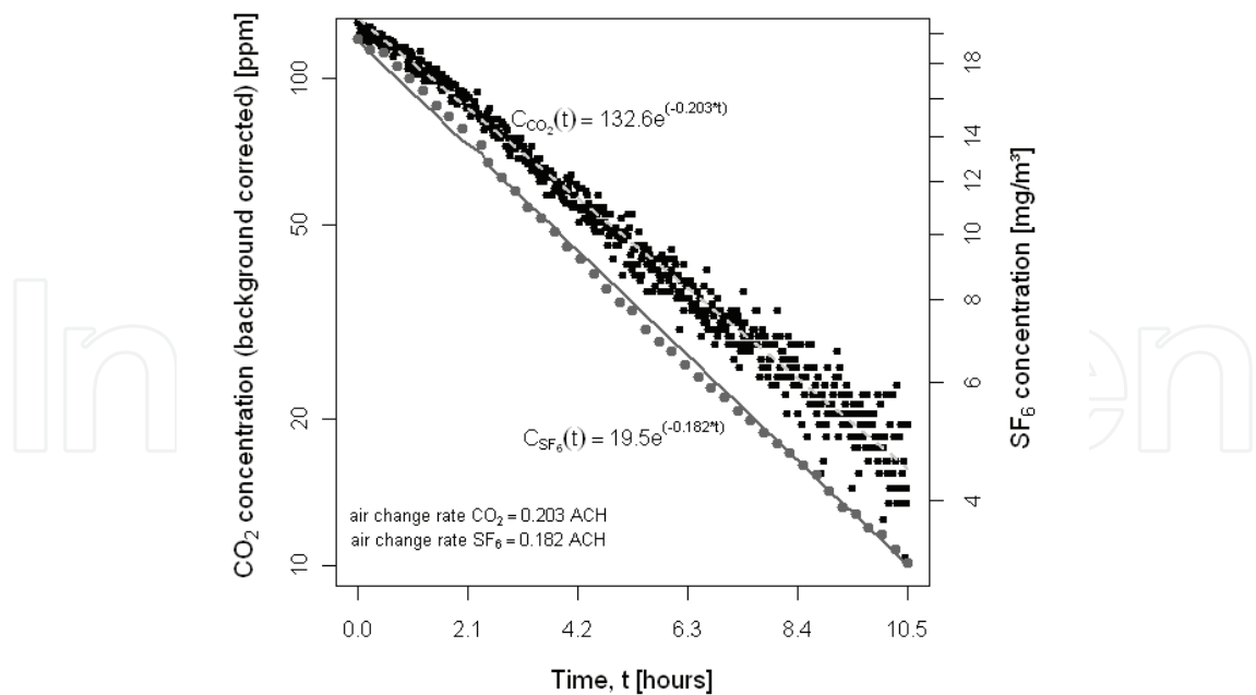
Fig. 9. Decay curves of CO 2 and sulphur hexafluoride (SF 6 ) and curve fits; simultaneous measurements in the same room.
