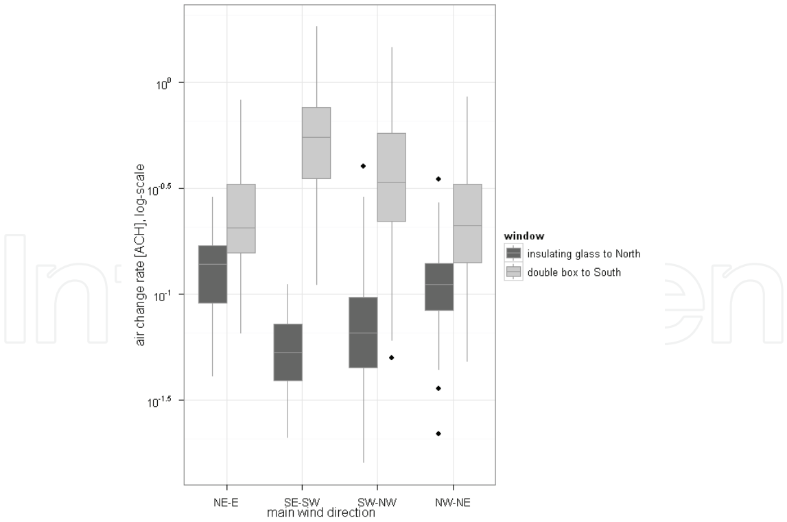
Fig. 12. Wind direction and ACR in office spaces equipped with windows of different construction. Windows and doors closed. Rooms with double box windows (A-D, F: n= 601), room with insulating glass window: n= 388).
