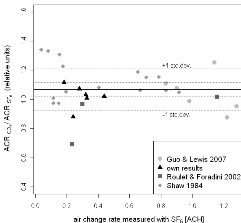
Fig. 10. Comparative air change determinations with CO 2 and SF 6 as tracer gases. Results from other authors and own results. Solid line: mean, dotted lines: 95% confidence interval of the mean, dashed lines: interval of \pm 1 standard deviation.
