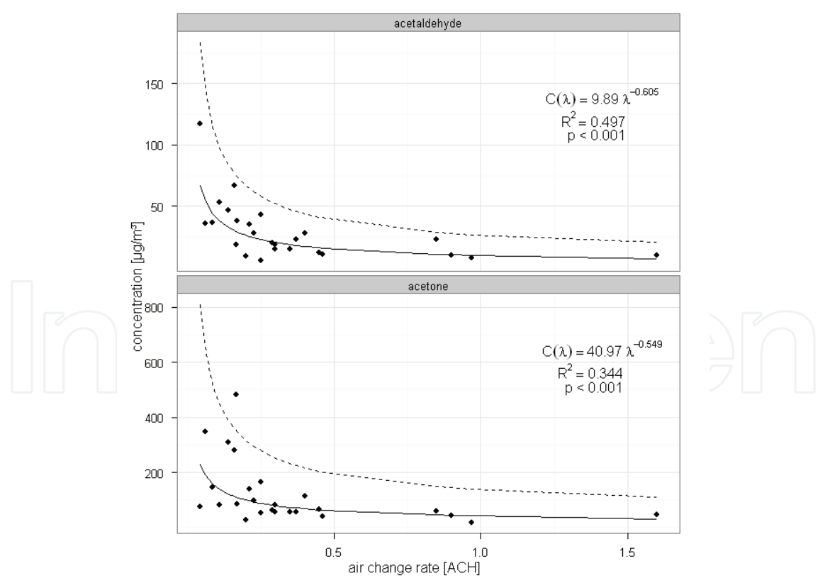
Fig. 17. a. and b. Concentrations of acetaldehyde (a) and acetone (b) and corresponding air change rates in rooms of the City of Berlin. Sampling: worst case conditions, solid line: mean concentration, dotted line: 90% prediction limit.
