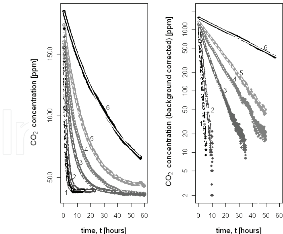
Fig. 5. CO 2 decay curves (black) in 6 rooms of different air tightness. White curves show results of regression analyses; a, nonlinear regression; b, linear regression of logarithmic values
