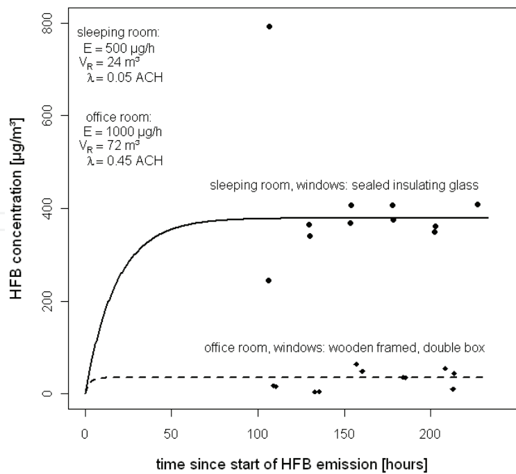
Fig. 8. Course of hexafluorobenzene concentration (HFB) in two rooms with different volumes and different window types, theoretical curves calculated from given emission rates E , air change rates \lambda , known room volumes V_R . Black glyphs: measured values.
