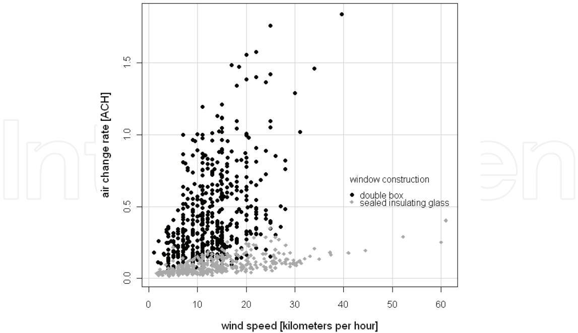
Fig. 11. Influence of wind speed on ACR in office spaces equipped with windows of different construction. Windows and doors closed. Rooms with double box windows (A-D, F: n= 611), room with insulating glass window: n= 388).
